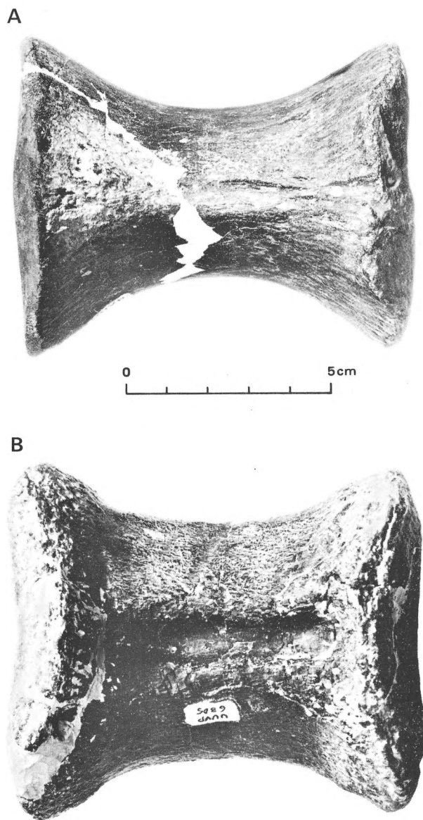
Figure 8. Caudal vertebrae of Allosaurus fragilis (A, UUV 6625) and Ceratosaurus sp. (B, UUV 6305).
