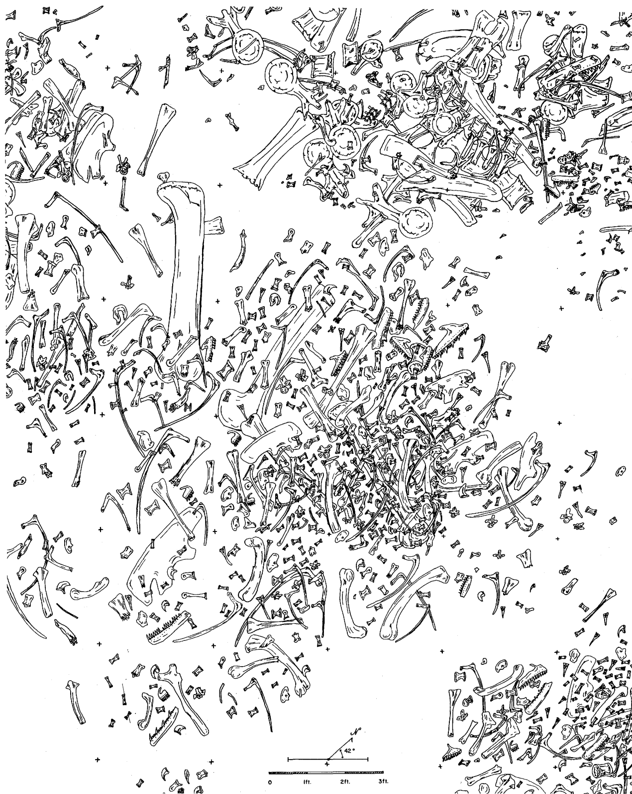
Figure 2. Section of composite map of the Cleveland-Lloyd Dinosaur Quarry, University of Utah Cooperative Dinosaur Project. Map compiled in August 1967 from quarry activity, 1960 through 1964.
