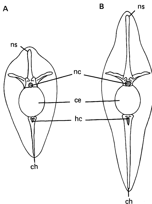
Figure 21. Anterior view of outlines at the base of the tails of Allosaurus (A) and Ceratosaurus (B). Abbreviations: ce—centrum, ch—chevron, hc—haemal canal, nc—neural canal, ns—neural spine.
