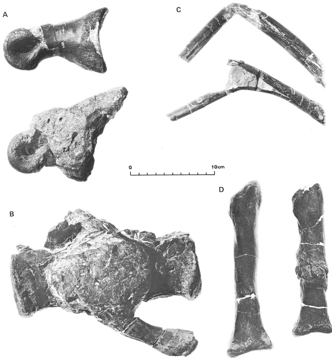
Figure 4. Bones of Allosaurus fragilis showing representative pathologies in the Cleveland-Lloyd Dinosaur Collection. Normal (UUVP 40-100) and abnormal (UUVP 1657) proximal phalanges, D-III, left pes (A); fused midcaudal vertebrae (UUVP 3771) and chevron (B); ribs with willow breaks (C); and normal (UUVP 86) and fractured (UUVP 687) right radii (D).
