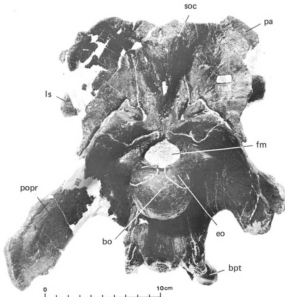
Figure 13. Posterior view of braincase (UUVP 5583) of Allosaurus fragilis . Abbreviations: bo—basioccipital, bpt—basipterygoid process, eo—exoccipital, fm—foramen magnum, ls—laterosphenoid, pa—parietal, popr—paroccipital process, soc—supraoccipital.
