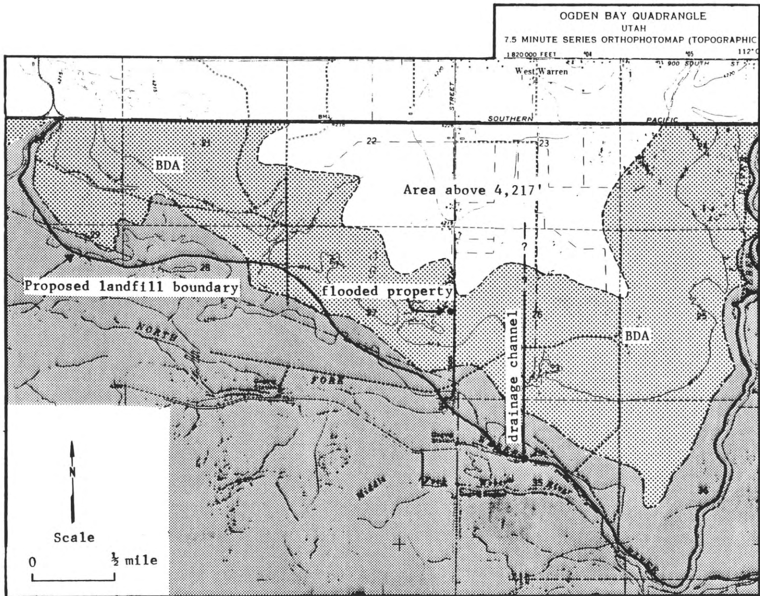
Figure 5. Proposed landfill site showing flooded property (●), drainage channel, Beneficial Development Area (BDA) of the Great Salt Lake (▨), and 100-year flood hazard zone of the Weber River (▨).
