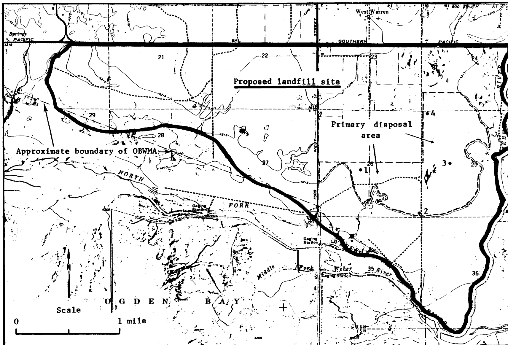
Figure 2. Proposed landfill site showing primary disposal area and test pit locations.
