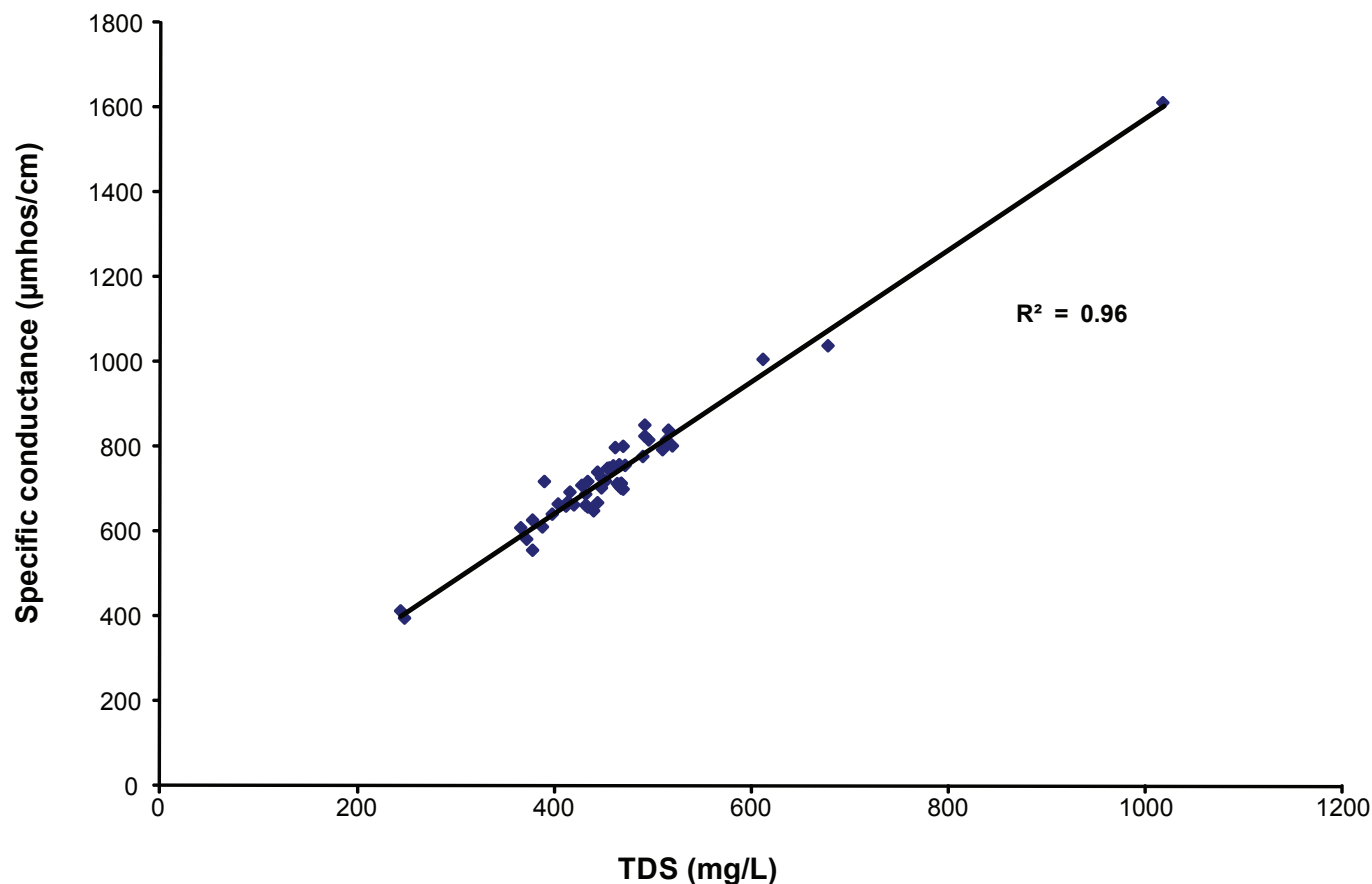
Figure 27. Specific conductance versus total-dissolved-solids concentration data for 50 wells in Morgan Valley, Morgan County, Utah. R -squared is 0.96. Based on Hem's (1985) equation for estimating TDS from specific conductance: KA=S , where K =specific conductance, S =TDS, A ranges from 0.55 to 0.96. The average A=0.63 (slope) was used to compute TDS in Morgan Valley.
