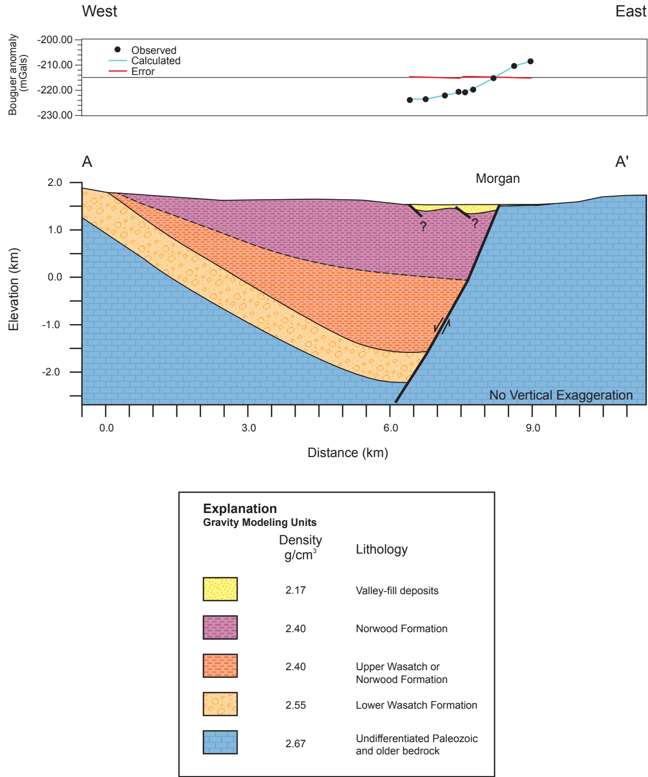
Figure 13. Gravity data and model cross section A–A' for traverse along Young Street in Morgan City. See figure 3 for traverse location. Cross section extrapolated to east and west based on geologic mapping and water-well logs.
