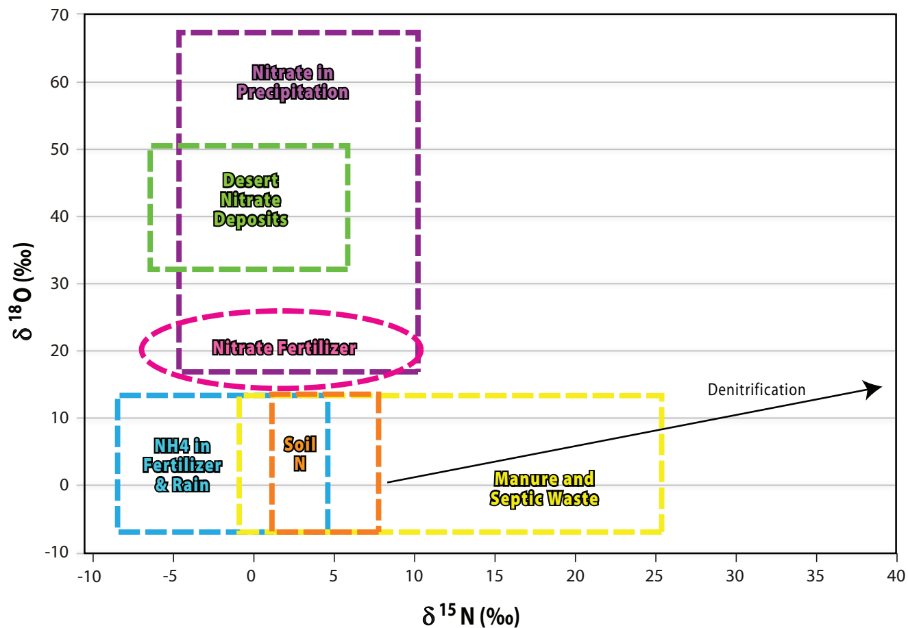
Figure 5. Plot of nitrogen and oxygen isotopes characterizing sources of nitrate (from Kendall, 1998).
