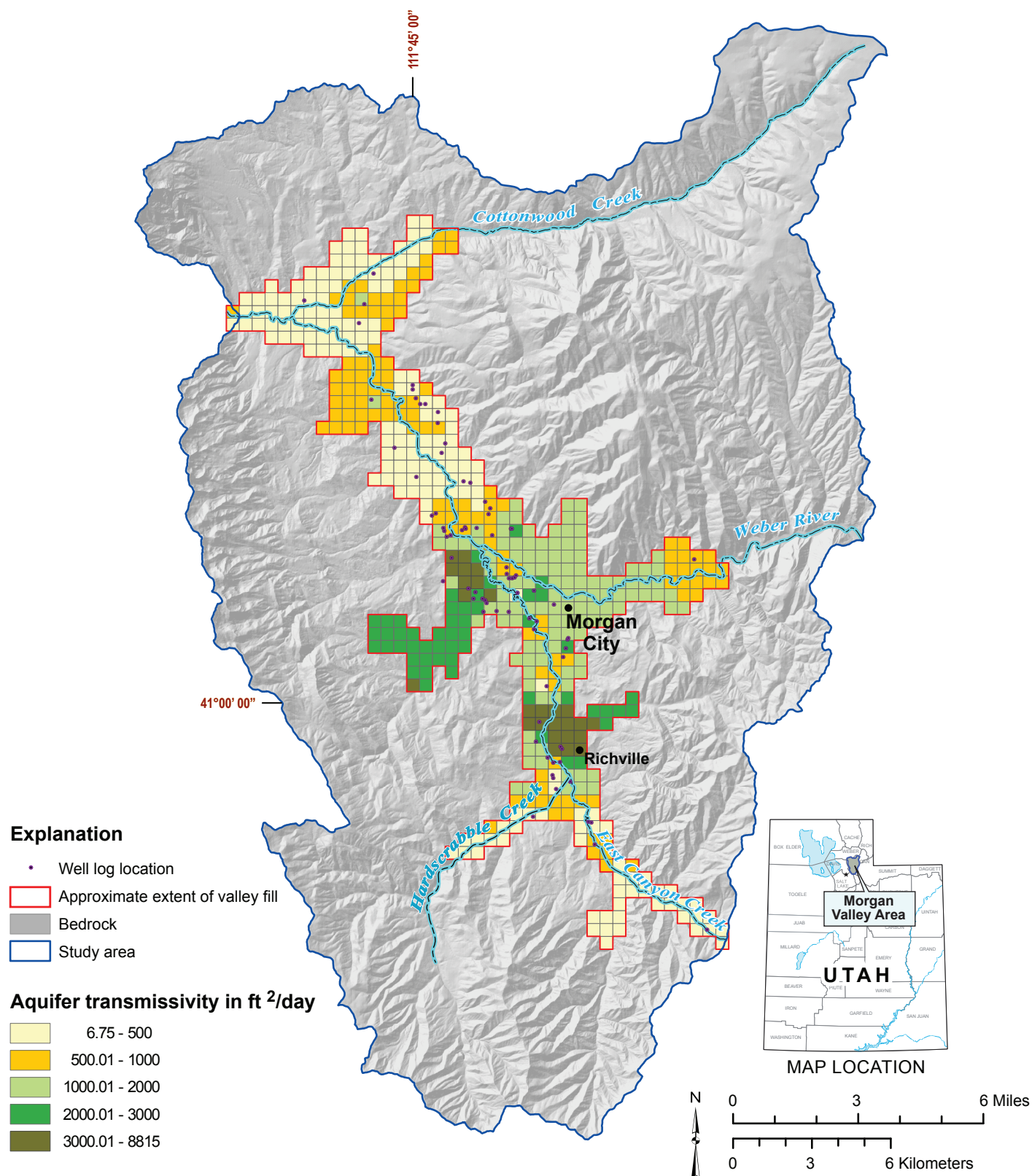
Figure 17. Valley-fill aquifer transmissivity (feet 2 /day) in Morgan Valley, Morgan County, Utah (transmissivity was estimated following TGUESS spreadsheet algorithm of Bradbury and Rothschild [1985] that applies the Cooper-Jacob approximation of the Theis equation).
