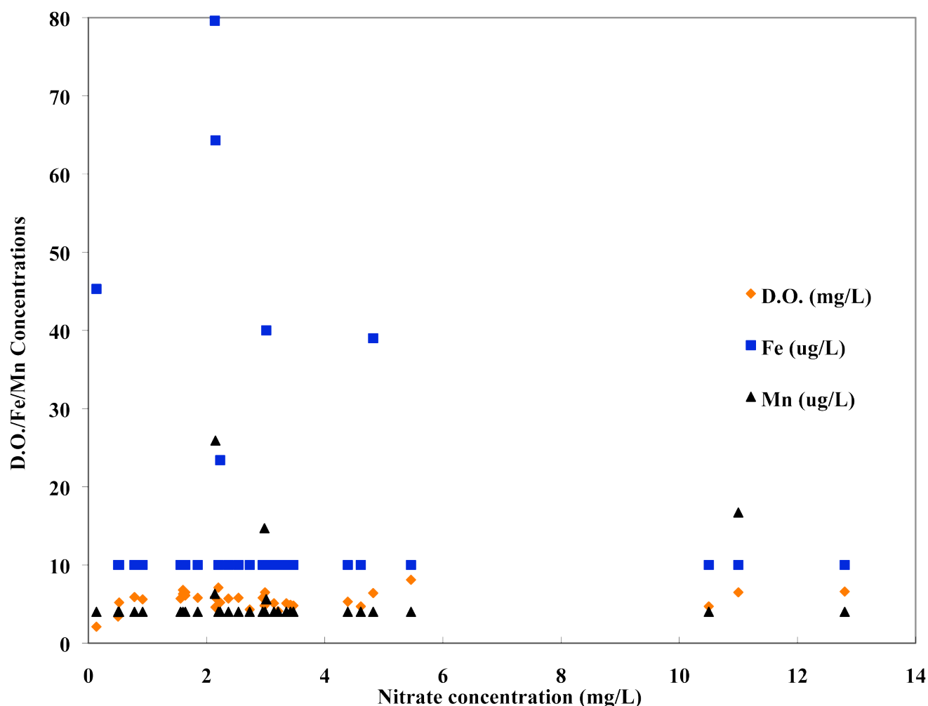
Figure 32. Nitrate concentration versus dissolved oxygen (D.O.), iron (Fe), and manganese (Mn) for water wells in Morgan Valley, Morgan County, Utah. An increase in Fe and Mn and a decrease in D.O. with decreasing nitrate indicates denitrification; this trend is not shown by our data.
