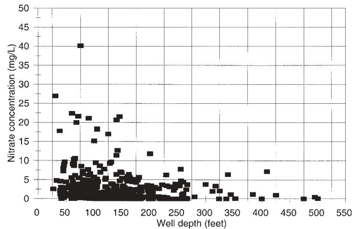
Figure 15. Well depth versus nitrate concentration, Sanpete Valley, Sanpete County, Utah. Correlation coefficient is -0.16 (R-squared is 0.026).
