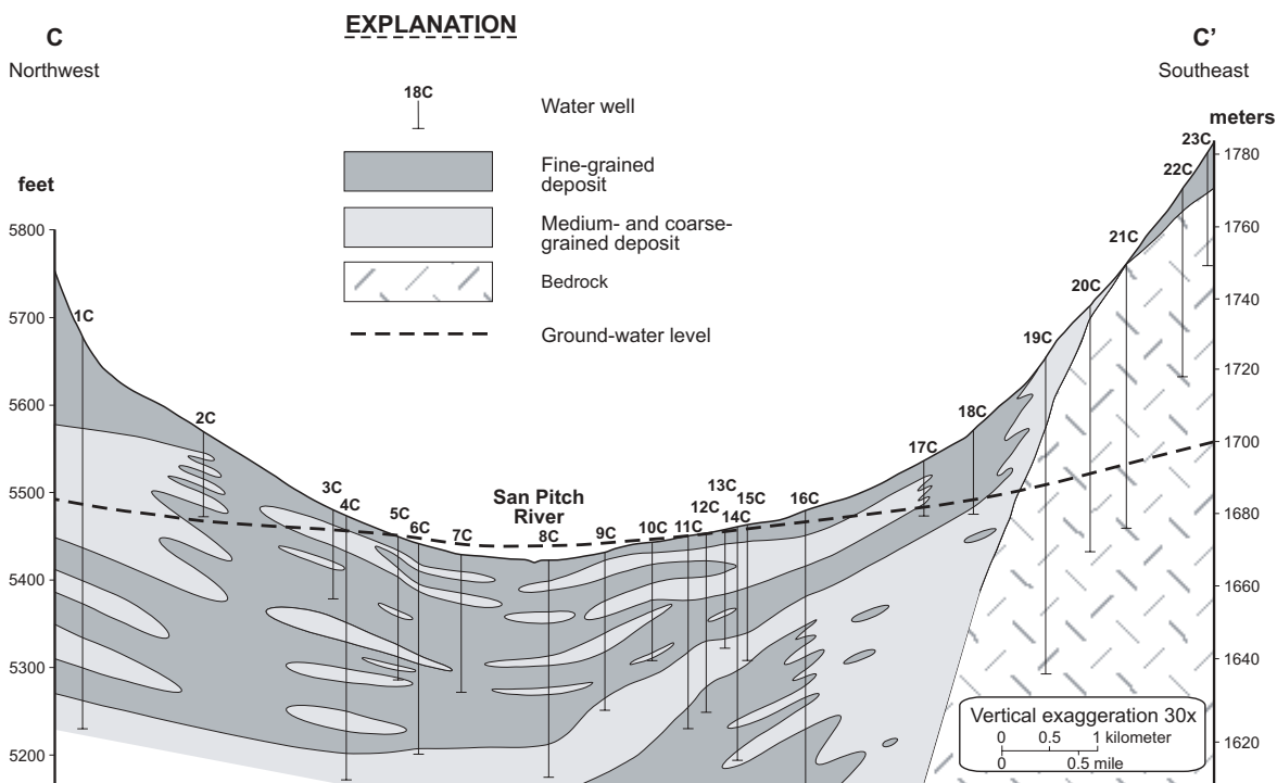
Figure C3. Diagrammatic cross section showing stratigraphy in the valley-fill deposits near Ephriam, Sanpete Valley, Sanpete County, Utah. Location of cross section is shown in figure 5.
