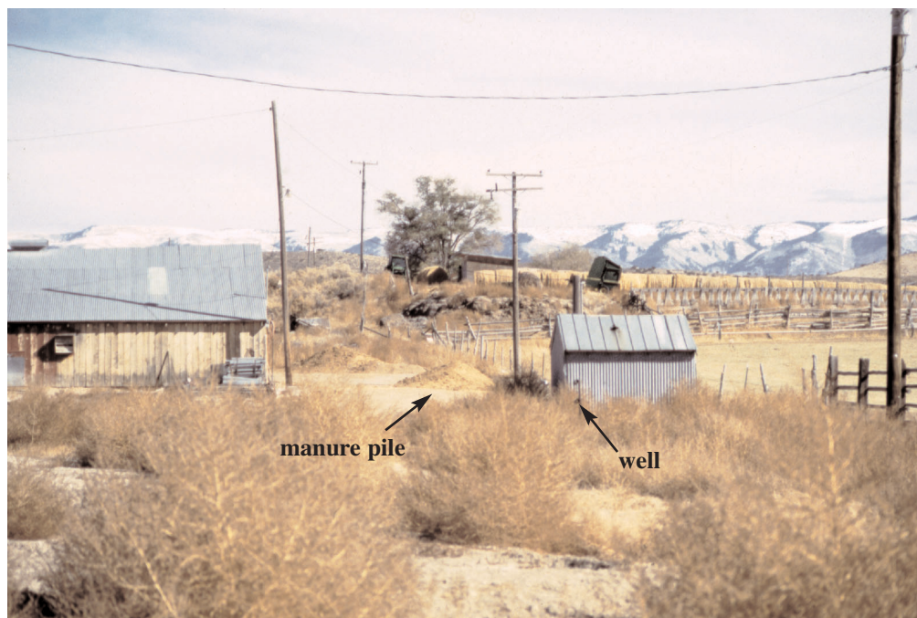
Figure 32. Example of turkey manure pile near a well having a high nitrate concentration in Sanpete Valley, Sanpete County, Utah.
