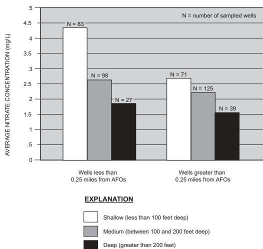
Figure 17. Average nitrate concentration for shallow, medium, and deep perforation-depth intervals for water wells less than or equal to 0.25 miles (0.4 km) and greater than 0.25 miles (0.4 km) from existing or former animal feed-lot operations (AFOs) in Sanpete Valley, Sanpete County, Utah.
