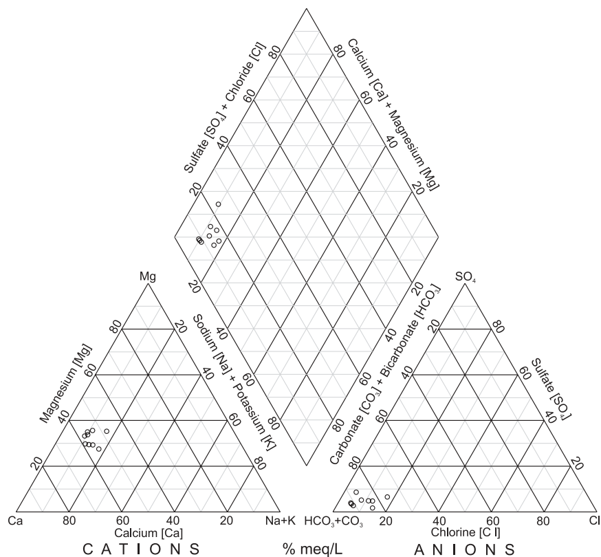
Figure 21. Piper plot of ground-water chemistry from wells north of Moroni in Sanpete Valley, Sanpete County, Utah.
