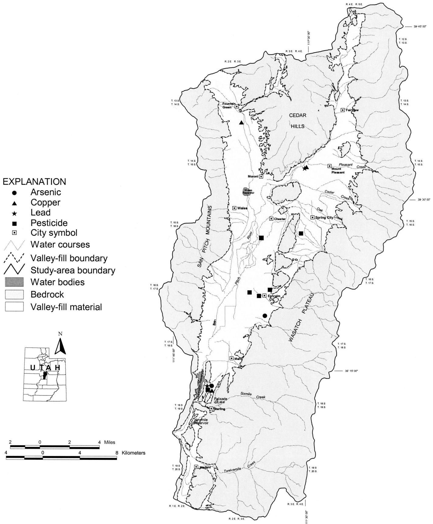
Figure 19. Distribution of wells having ground-water constituents that exceed water-quality standards, and pesticides above maximum reporting level but below water-quality standards in Sanpete Valley, Sanpete County, Utah..
