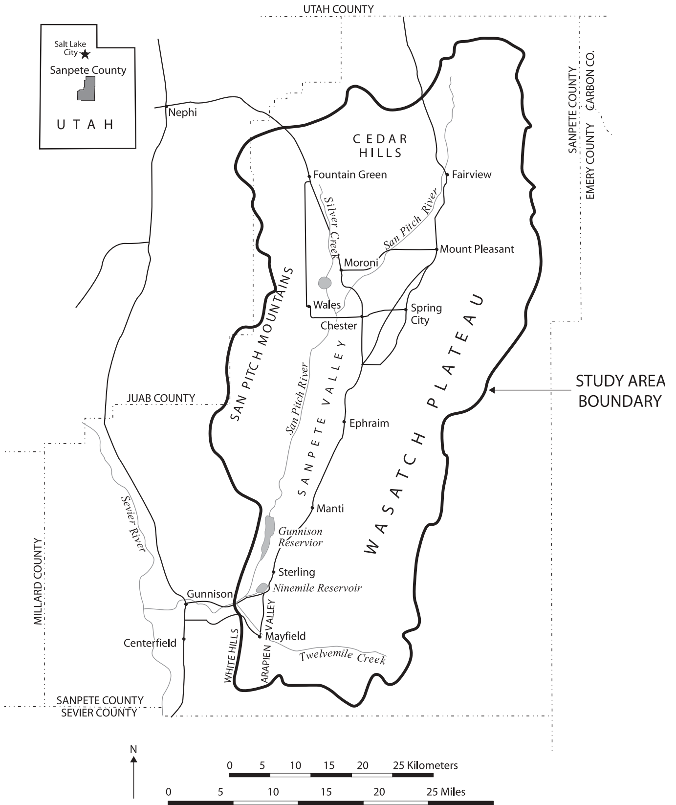
Figure 1. Sanpete Valley, Sanpete County, Utah study area.
