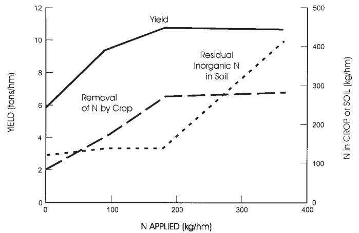
Figure 31. Yield, removal of nitrogen by crop, and residual nitrogen in soil after harvest at different nitrogen fertilizer application rates (from National Academy of Sciences, 1978).
