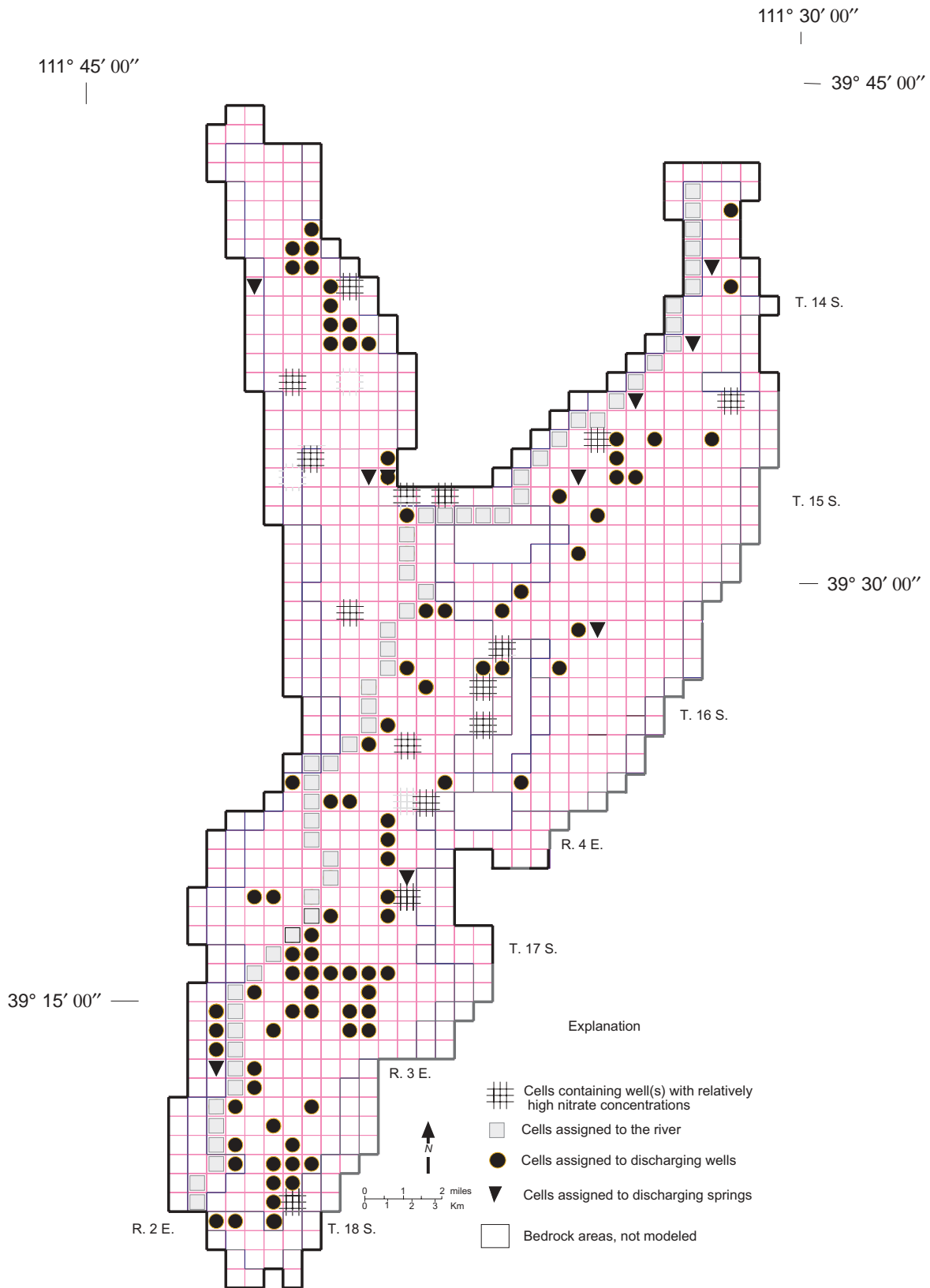
Figure 30. Location of cells that represent wells with high nitrate concentrations. Also shown are cells that represent discharging wells and springs, and river.
