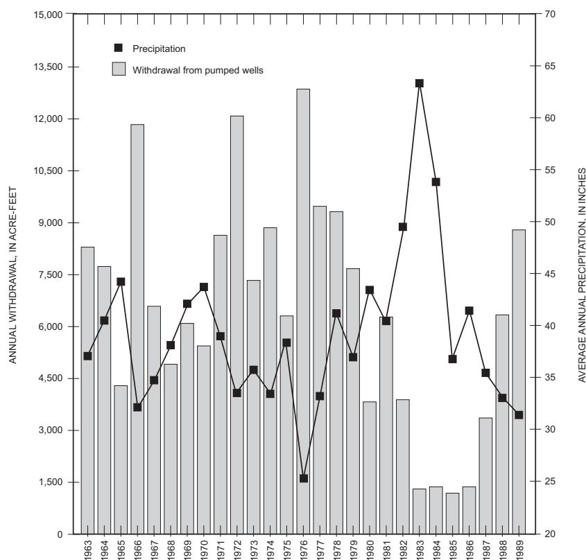
Figure C4. Annual ground-water withdrawals from pumped wells in Sanpete Valley, Sanpete County, Utah, versus precipitation at Meadows climatic station, Wasatch Plateau, Utah, calendar years 1963-1989 (from Wilberg and Heilweil, 1995).
