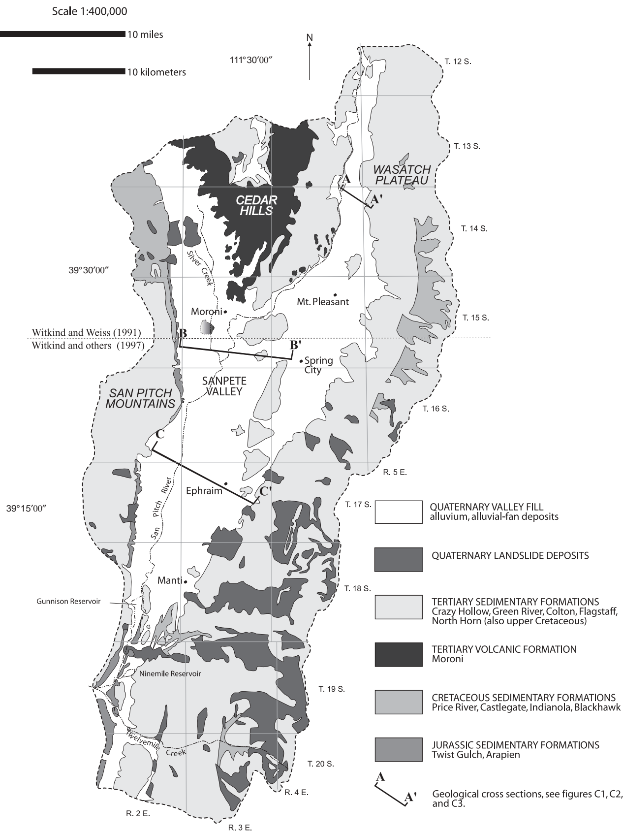
Figure 5. Simplified geology and sources of geologic mapping for Sanpete Valley, Sanpete County, Utah. See plate 3A for a more detailed geologic map.
