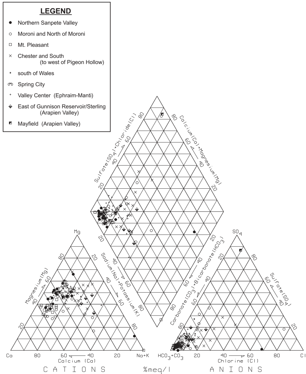
Figure 8. Piper plot showing overall ground-water chemistry from water wells sampled in this study; the water is dominantly calcium-magnesium-bicarbonate type for Sanpete Valley, Sanpete County, Utah. Different symbols correspond to different areas throughout the valley.
