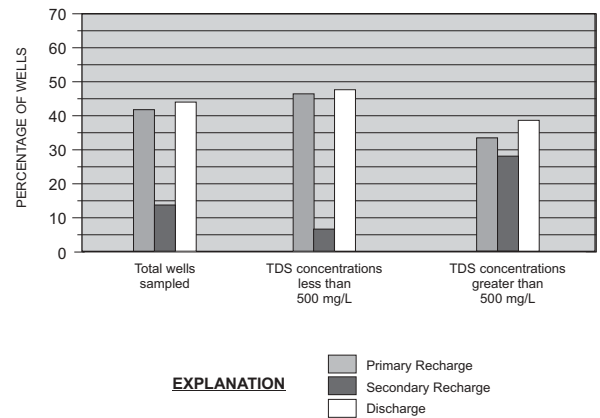
Figure 12 Percentage of wells in hydrogeologic setting sampled for total-dissolved-solids (TDS) concentrations in primary and secondary recharge and discharge areas that are less than 500 mg/L and greater than 500 mg/L in Sanpete Valley, Sanpete County, Utah. This shows higher TDS concentrations are present in all hydrogeologic settings and that location in hydrogeologic setting does not seem to affect TDS concentrations.
