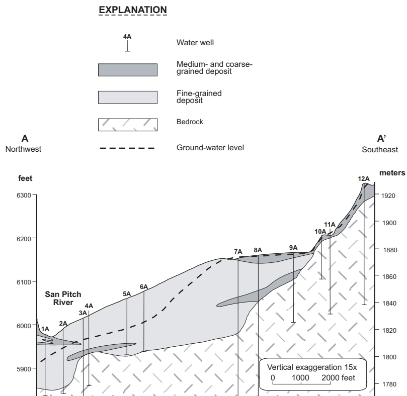
Figure C1. Diagrammatic cross section showing stratigraphy in the valley-fill deposits north of Fairview, Sanpete Valley, Sanpete County, Utah. Location of cross section is shown in figure 5.
