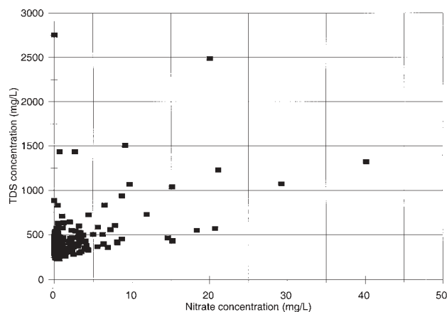
Figure 18. Nitrate concentration versus total-dissolved-solids (TDS) concentration for ground water for 118 wells in Sanpete Valley, Sanpete County, Utah. Correlation coefficient is 0.4 (R-squared is 0.016).
