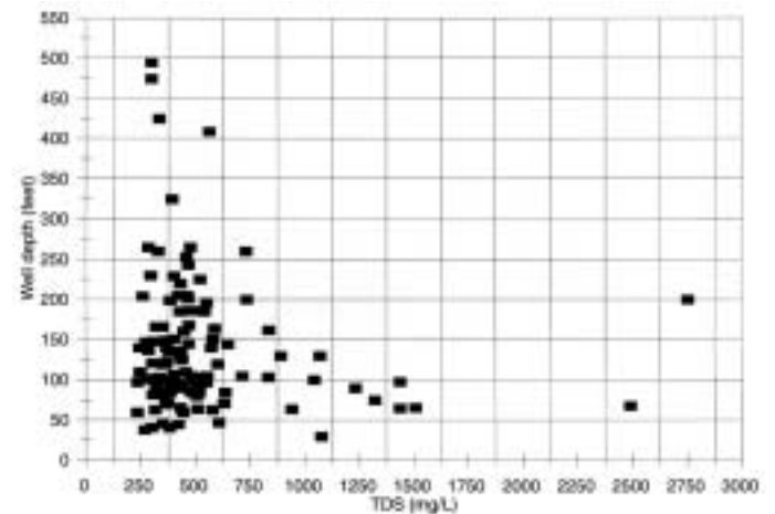
Figure 11. Relationship between well depth and total-dissolved-solids (TDS) concentrations in Sanpete Valley, Sanpete County, Utah. Correlation coefficient is -0.12 (R-squared is 0.014).
