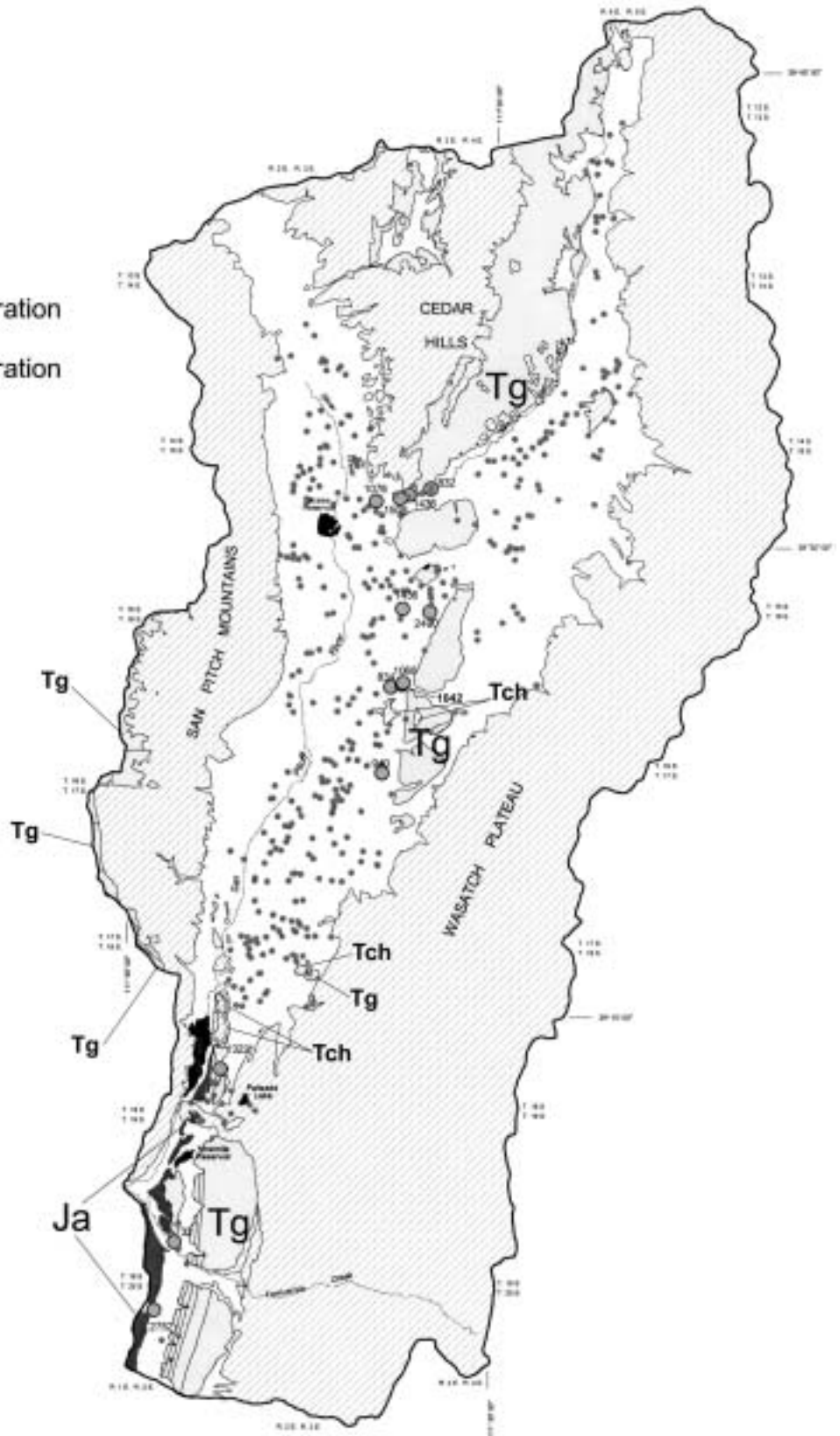
Figure 13. Distribution of elevated total-dissolved-solids-concentration wells and adjacent rock types (Jurassic Arapien Shale and Tertiary Green River and Crazy Hollow Formations) in Sanpete Valley, Sanpete County, Utah.
