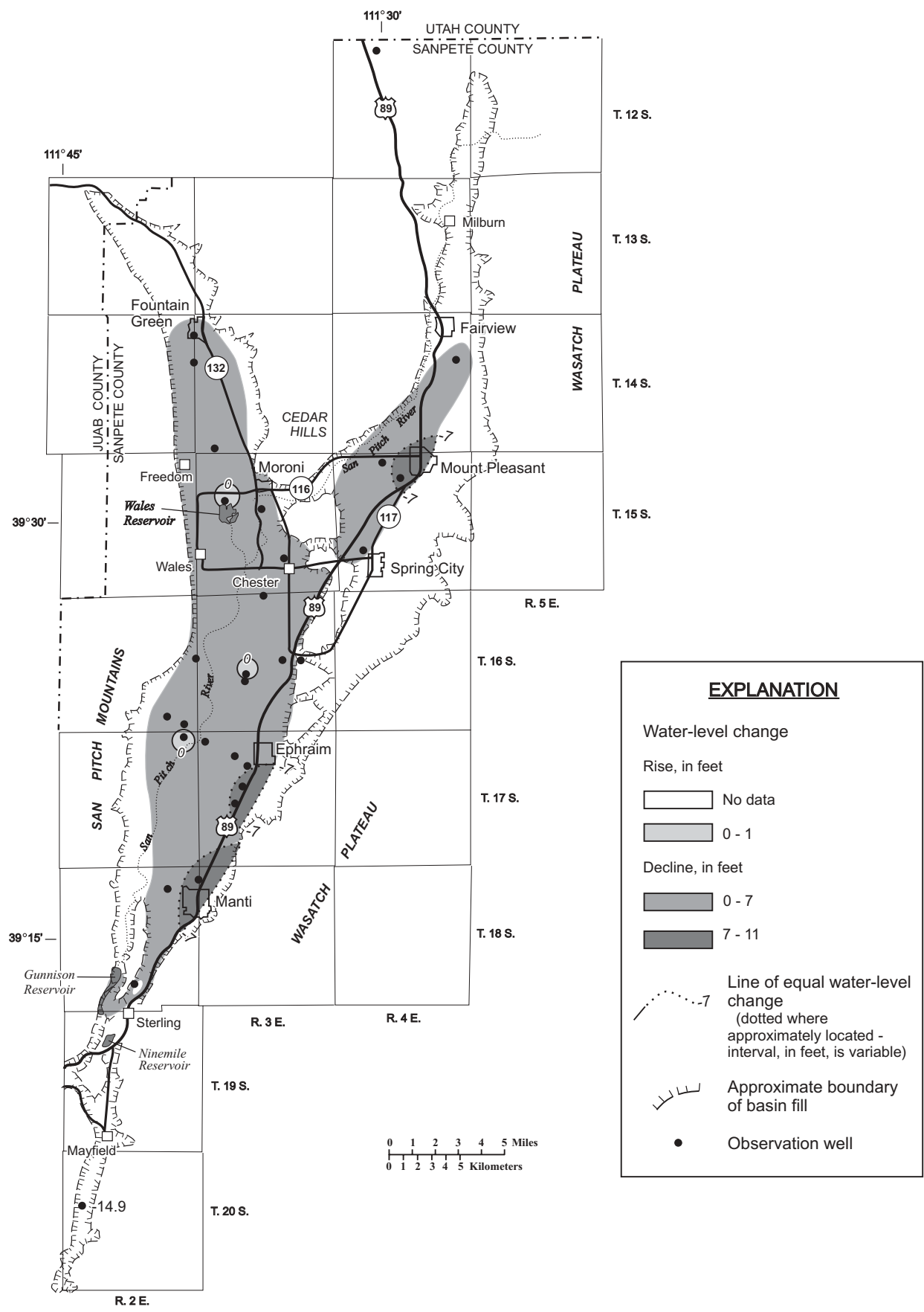
Figure C5. Change in water levels from March 1970 to March 2000, Sanpete Valley, Sanpete County, Utah (modified from Burden and others, 2000).
