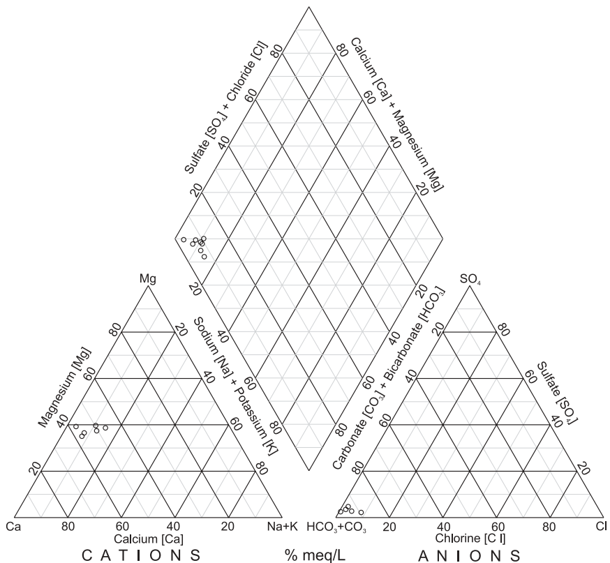
Figure 22. Piper plot of ground-water chemistry from wells near Mount Pleasant in Sanpete Valley, Sanpete County, Utah.
