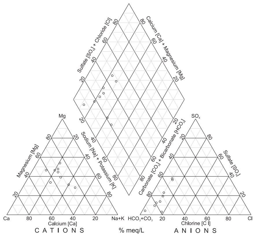
Figure 24. Piper plot of ground-water chemistry from wells in Moroni proper in Sanpete Valley, Sanpete County, Utah.
