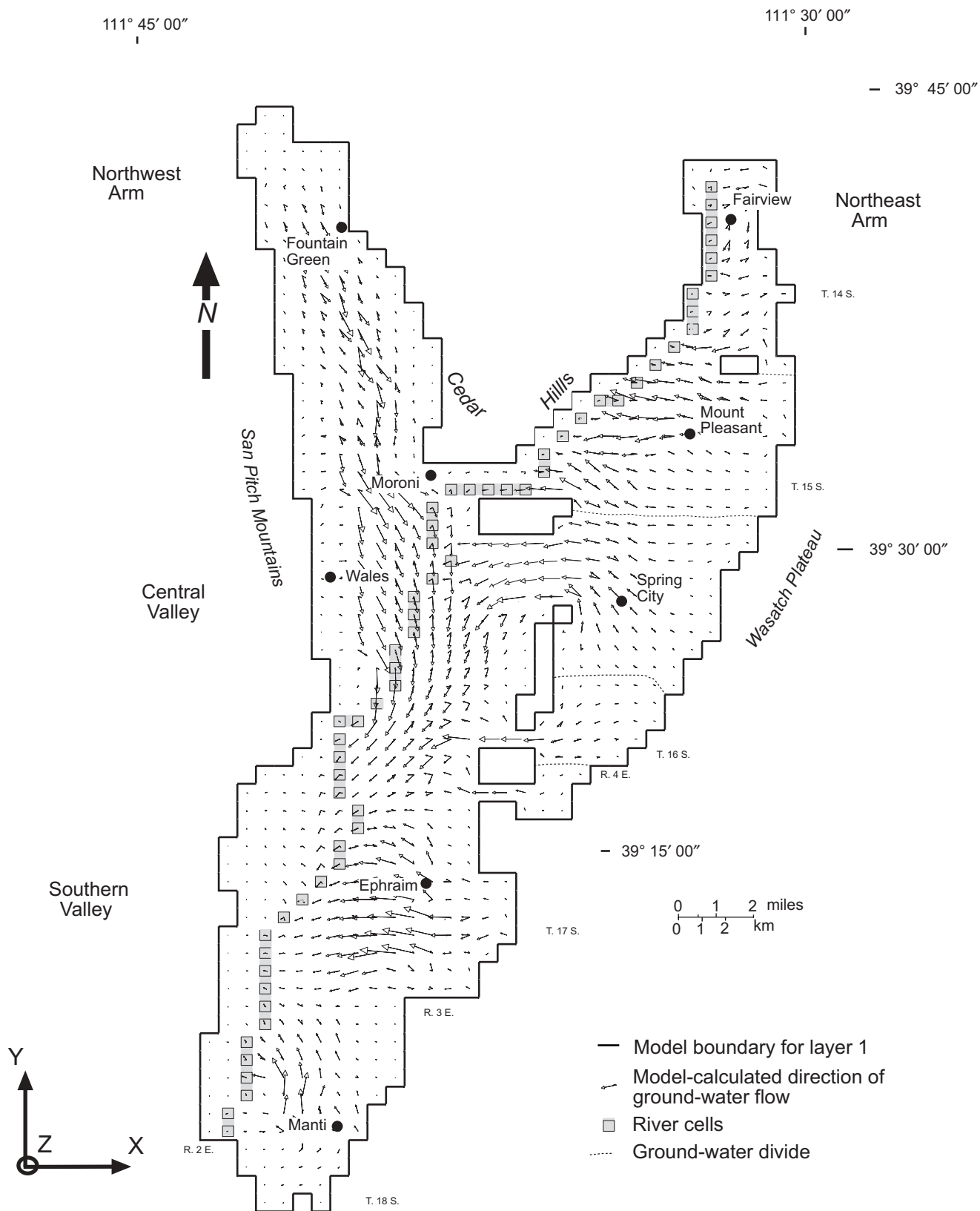
Figure 28. Model-calculated ground-water flow directions and relative magnitude (indicated by the length of the arrow) for each element on the basis of the steady-state simulation. The flow vectors determine the regional flow pattern for Sanpete Valley, Sanpete County, Utah.
