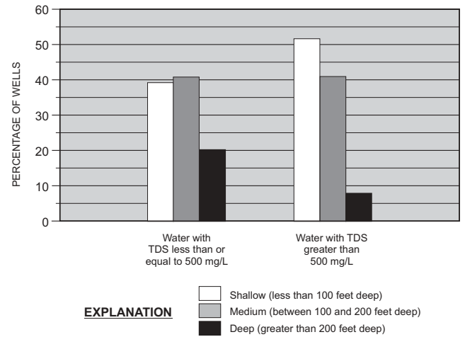
Figure 10. Percentage of wells in shallow-, medium-, and deep-perforated intervals above and below 500 mg/L total-dissolved-solids (TDS) concentrations in Sanpete Valley, Sanpete County, Utah. Note shallow wells generally have higher TDS.
