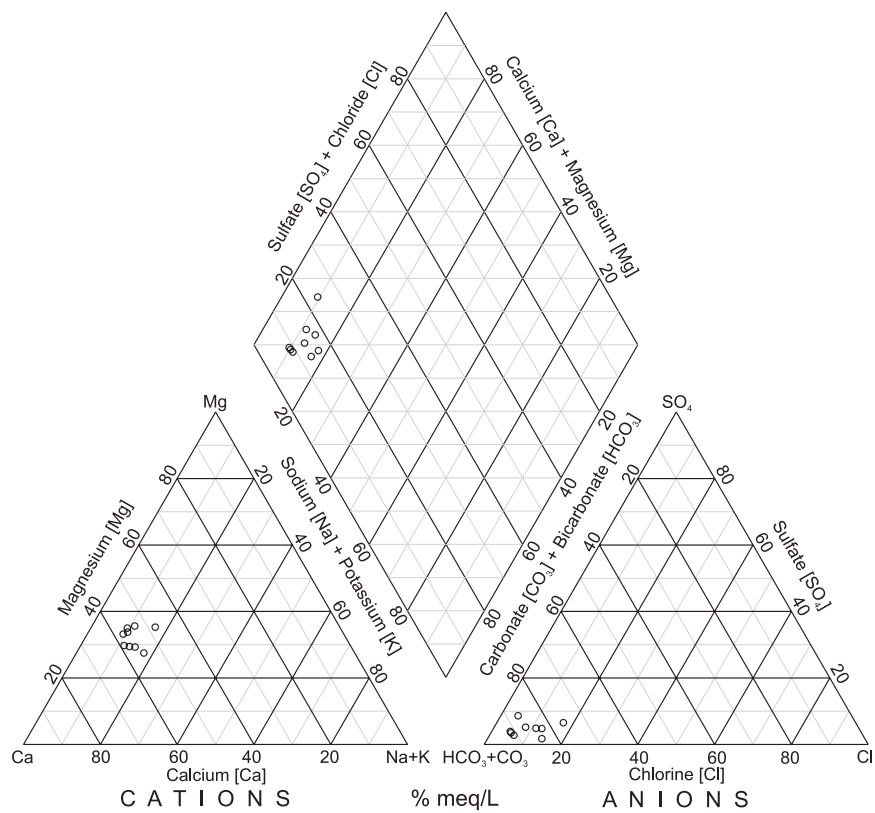
Figure 23. Piper plot of ground-water chemistry from wells west of Moroni and south of Fountain Green in Sanpete Valley, Sanpete County, Utah.
