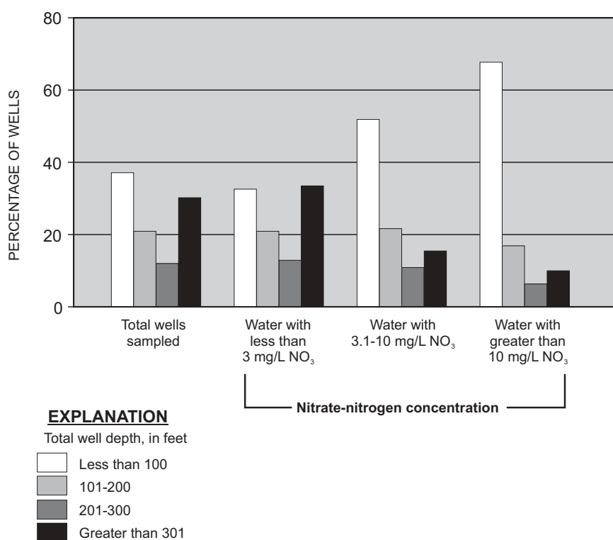
Figure D1. Distribution of nitrate concentrations (milligrams per liter) in well water with well depth. About 124,000 wells were included in the analysis (from Madison and Brunett, 1985).
