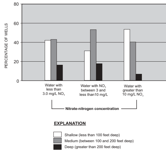
Figure 14. Percentage of wells in each shallow, medium, and deep perforation-depth interval that are less than 3 mg/L, between 3 and less than 10 mg/L, and greater than 10 mg/L nitrate concentration in Sanpete Valley, Sanpete County, Utah.
