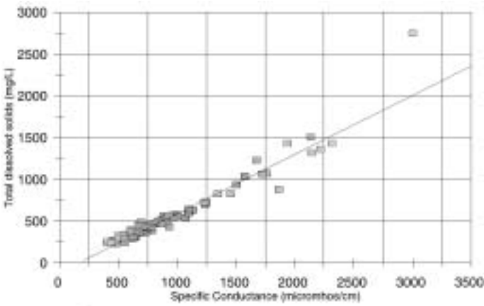
Figure 9. Relation of specific conductance to total-dissolved-solids concentrations in ground-water samples collected in Sanpete Valley, Sanpete County, Utah. Correlation coefficient is 0.97.
