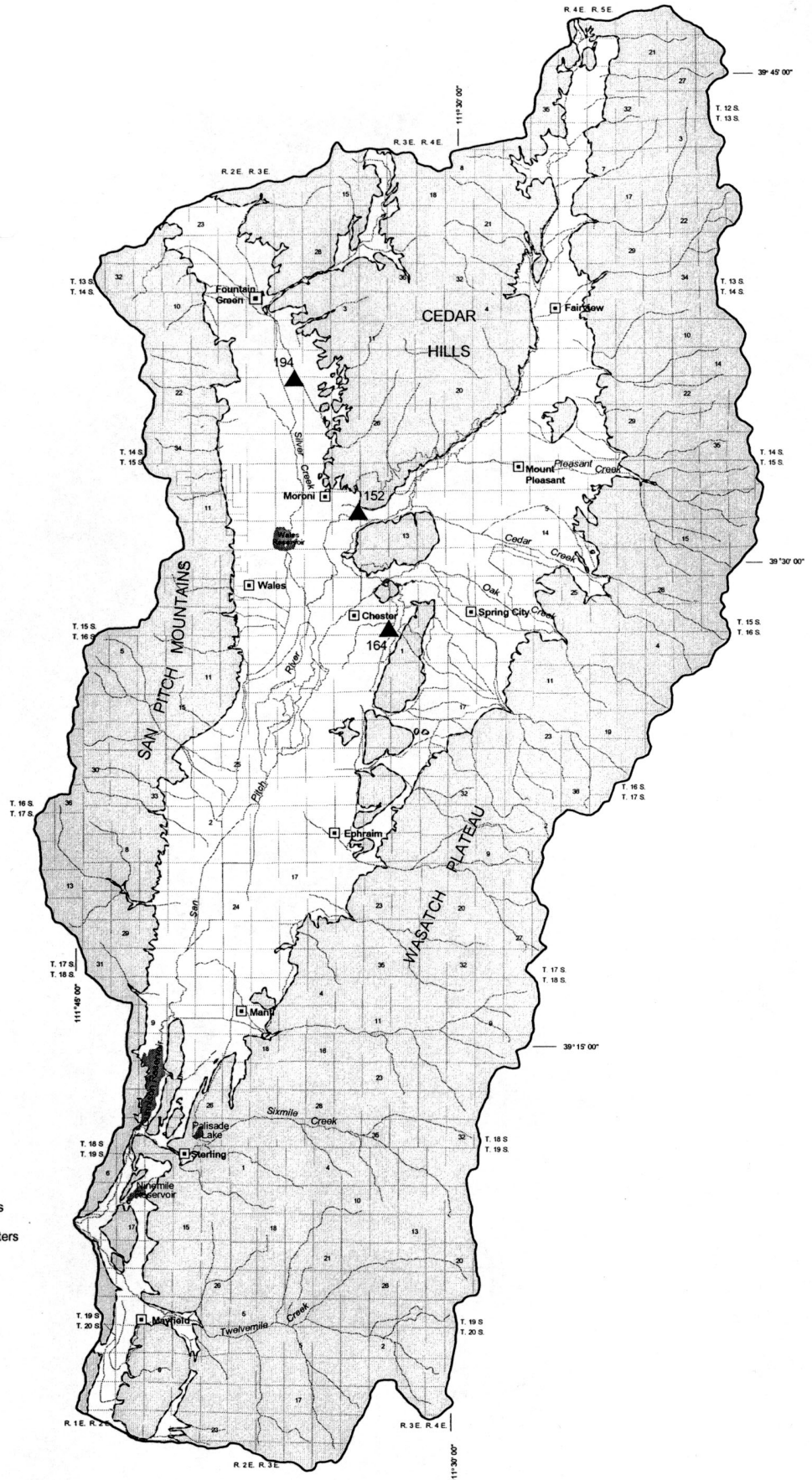
Figure 25. Location of wells sampled for tritium in Sanpete Valley, Sanpete County, Utah.
