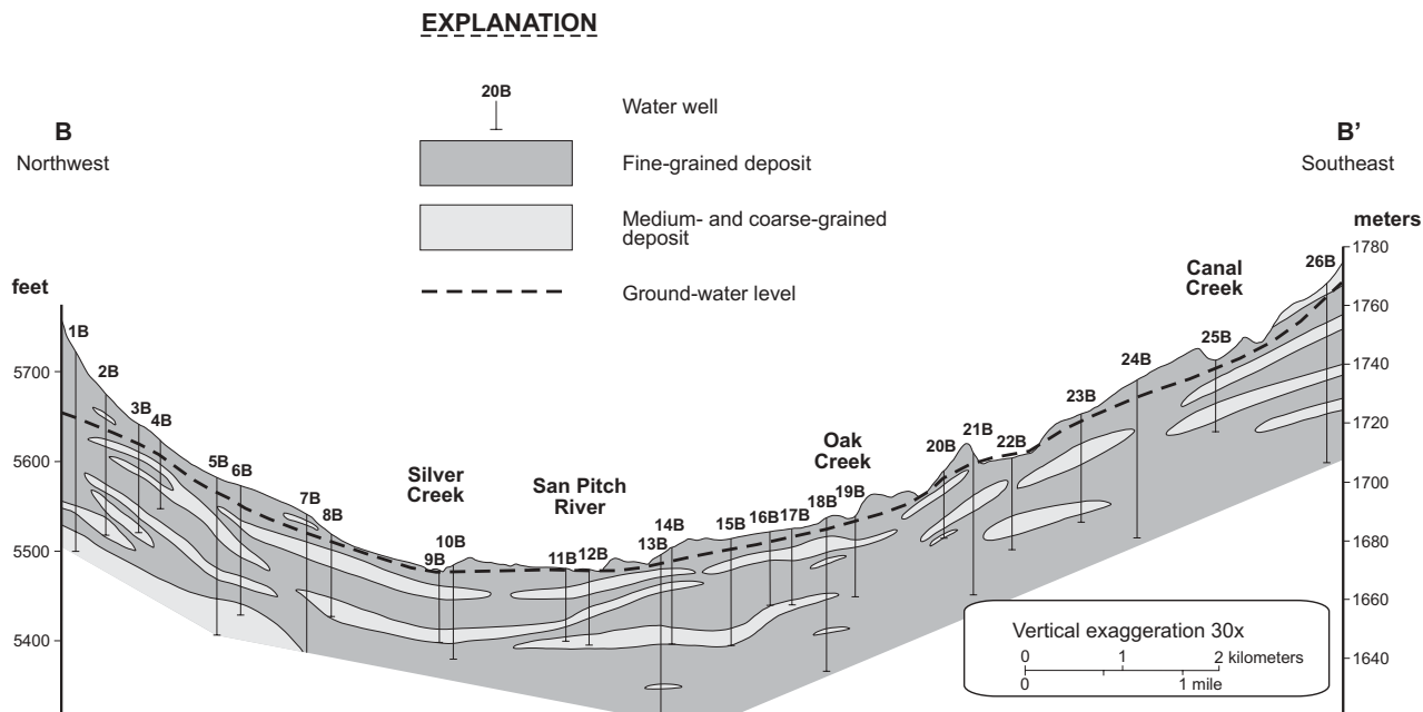
Figure C2. Diagrammatic cross section showing stratigraphy in the valley-fill deposits between Wales and Spring City, Sanpete Valley, Sanpete County, Utah. Location of cross section is shown in figure 5.
