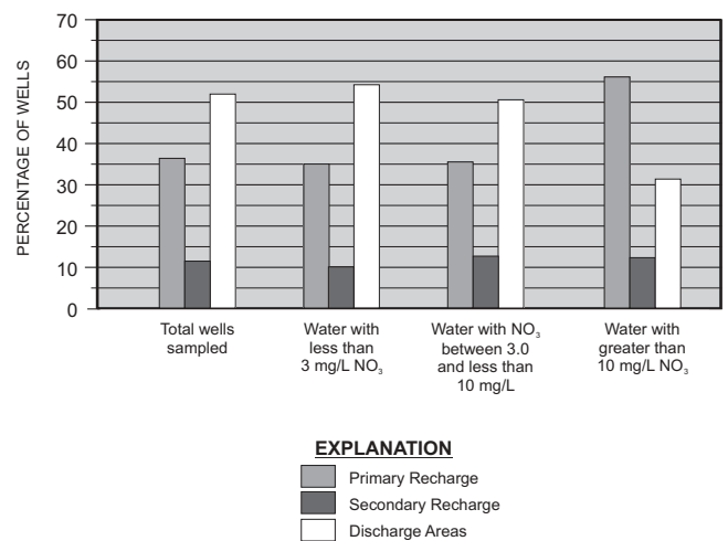
Figure 16. Percentage of wells in each hydrogeologic setting category that are less than 3 mg/L, between 3 and 10 mg/L, and greater than 10 mg/L nitrate concentration in Sanpete Valley, Sanpete County, Utah.
