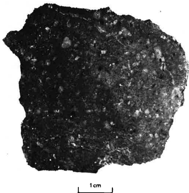
FIGURE 5. — Lower vitrophyre of Packard Quartz Latite from exposures 980 ft (299 m) S. 6° W. of Central Standard shaft. Same as sample 1, table 1. Dark phenocrysts are biotite; light phenocrysts are plagioclase and sanidine. Quartz phenocrysts are present but not distinguishable in photograph from obsidian matrix.
