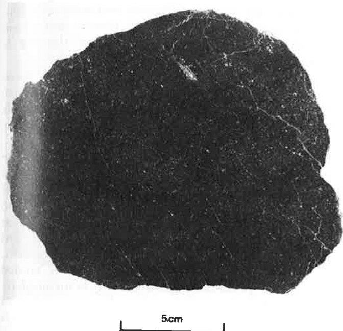
FIGURE 9. — Flow member of Copperopolis Latite from exposures 2,500 ft (762 m) S. 15° W. of Willow Spring. Same as sample 1, table 4. Light phenocrysts are all plagioclase.
