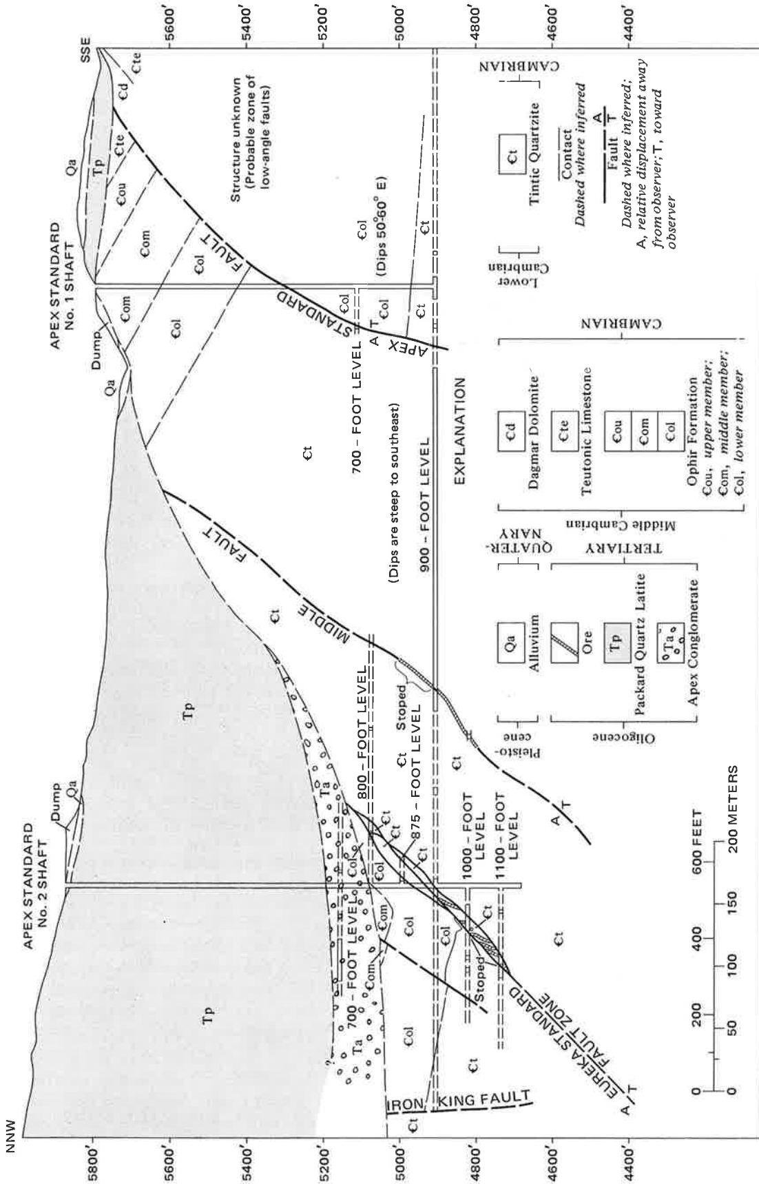
FIGURE 41. — Geologic cross section through Apex Standard No. 1 and No. 2 shafts.
