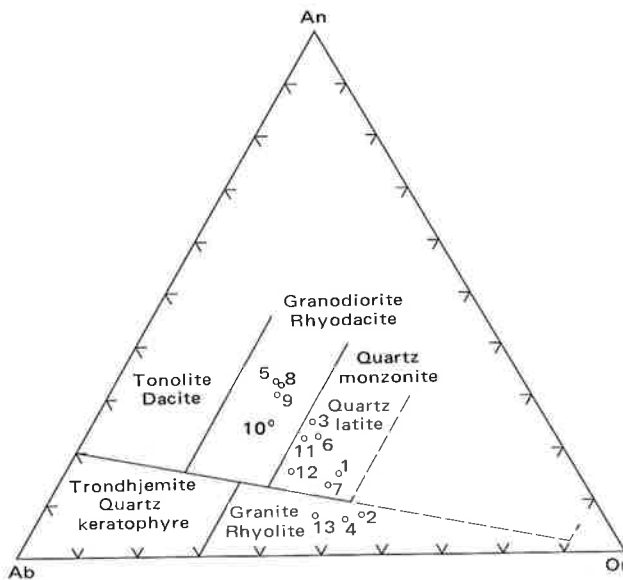
FIGURE 27. — Ternary diagram showing the normative feldspar content of averaged igneous rocks of the East Tintic Mountains. Samples 1-11 are from table 7; samples 12 and 13 are the same as samples 1 and 2 of table 6. Fields are from O'Connor (1965).
