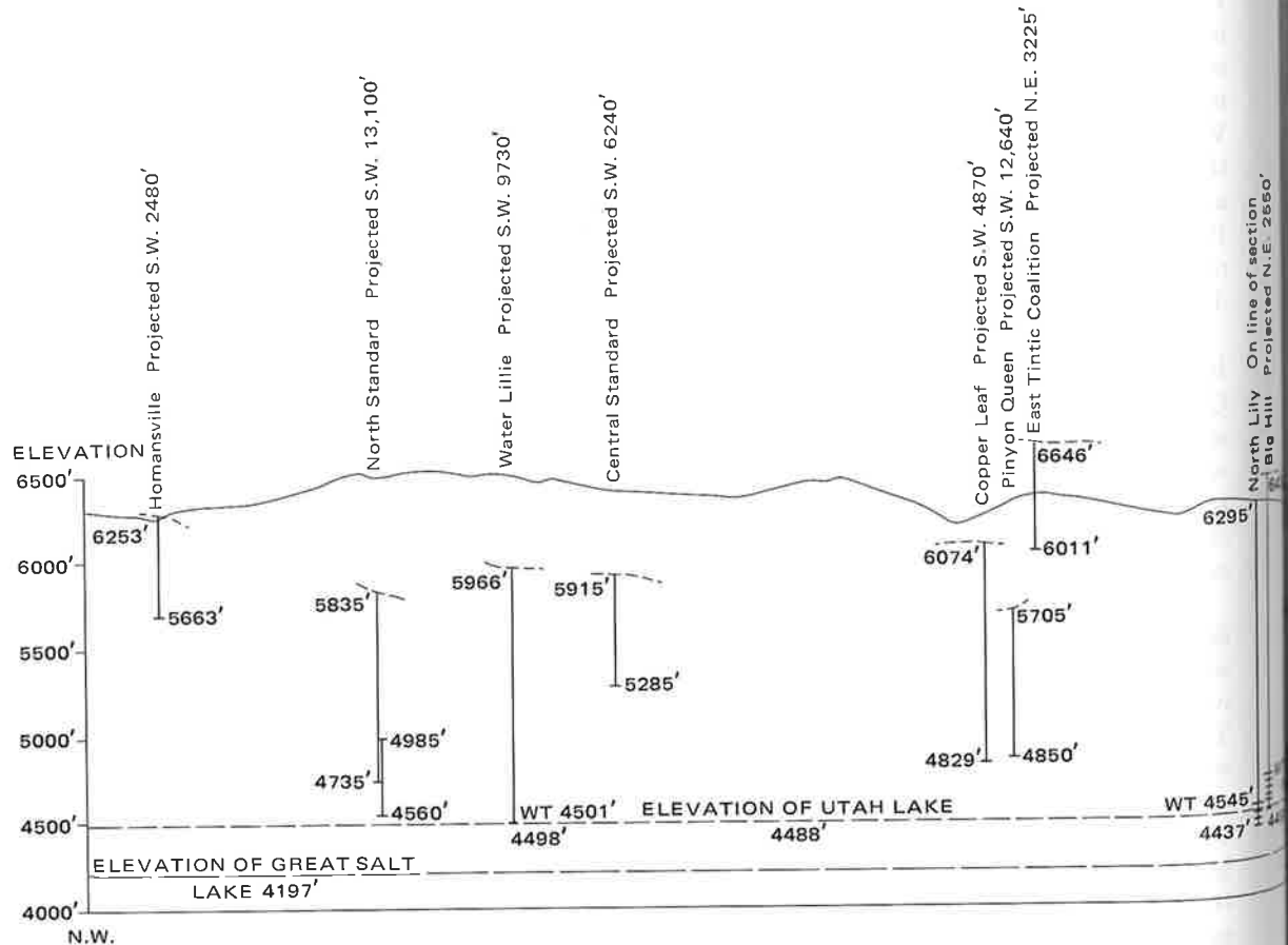
FIGURE 37. — Shafts and water table data, East Tintic district, Utah.
