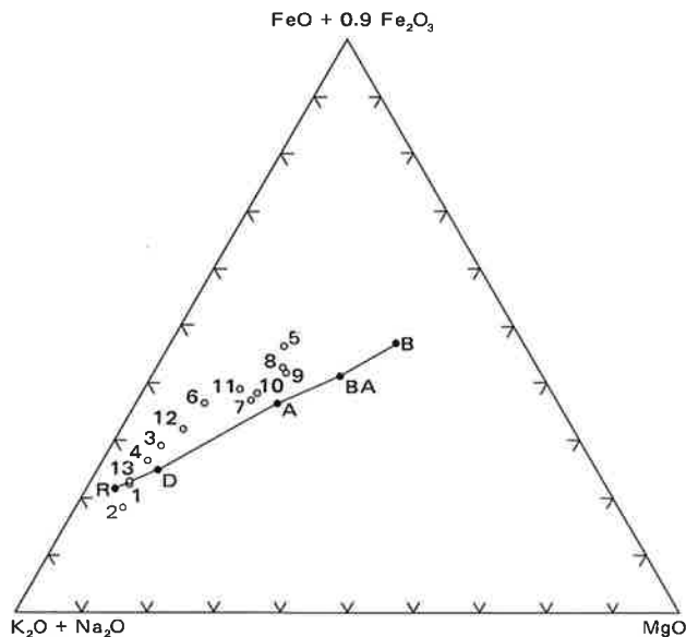
FIGURE 31. — Ternary diagram of alkalis ( \text{K}_2\text{O} + \text{Na}_2\text{O} ), iron oxide ( \text{FeO} + 0.9 \text{Fe}_2\text{O}_3 ), and magnesia in the igneous rocks of the East Tintic Mountains. Samples 1-11 from table 7; samples 12 and 13 are the same as samples 1 and 2 in table 6. Closed circles show average rhyolite (R), dacite (D), andesite (A), basaltic andesite (BA), and basalt (B) from the Cascade province (Carmichael, 1964, p. 448).
