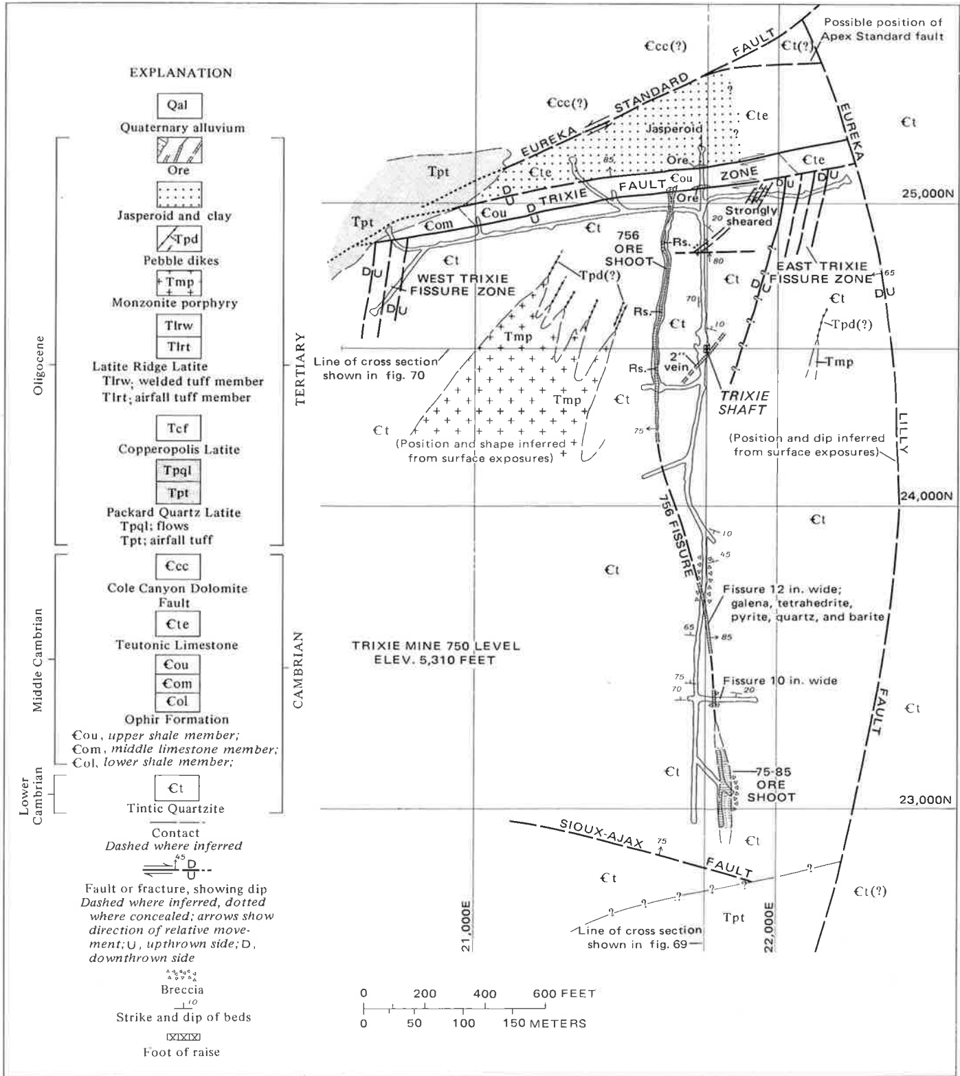
FIGURE 68. — Geologic plan of 750 level of Trixie mine.
