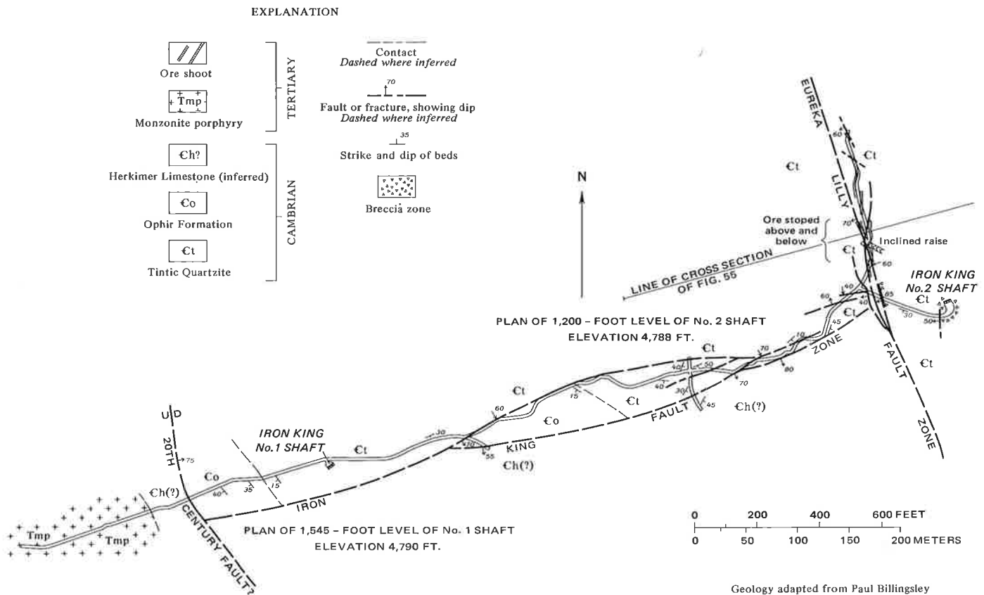
FIGURE 54. — Geologic plan of 1,545-ft level of Iron King Mine.
