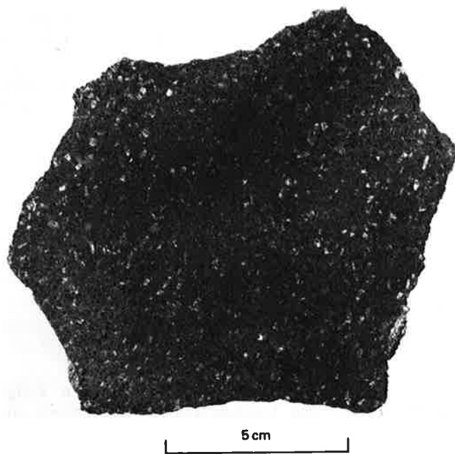
FIGURE 12. — Monzonite porphyry of the Gough sill 1,650 feet (503 m) S. 80° E. of Gold Bond Spring. Light phenocrysts are conspicuously zoned plagioclase; dark phenocrysts are chiefly biotite but also included augite and hypersthene.
