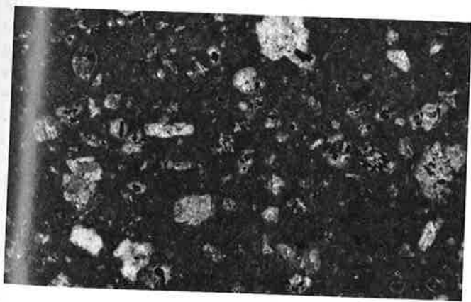
FIGURE 25. — Silver Shield Quartz Latite from flow unit exposed in railroad cut 2,200 ft (671 m) southeast of mouth of Pinyon Creek Canyon. Light phenocrysts include quartz (rounded, medium gray, fractured), sanidine (rectangular, medium gray, unfractured), and plagioclase (light gray to white). Dark phenocrysts visible in photograph are predominantly biotite. Same as sample 1, table 6.
