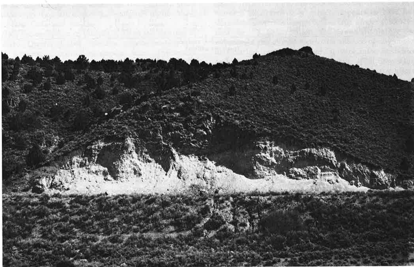
FIGURE 7. — Zone of accelerated weathering in Packard Quartz Latite in railroad cut 1,000 ft (305 m) east-southeast of Central Standard shaft. Unaltered lava overlying altered zone has an irregular but sharp lower contact.
