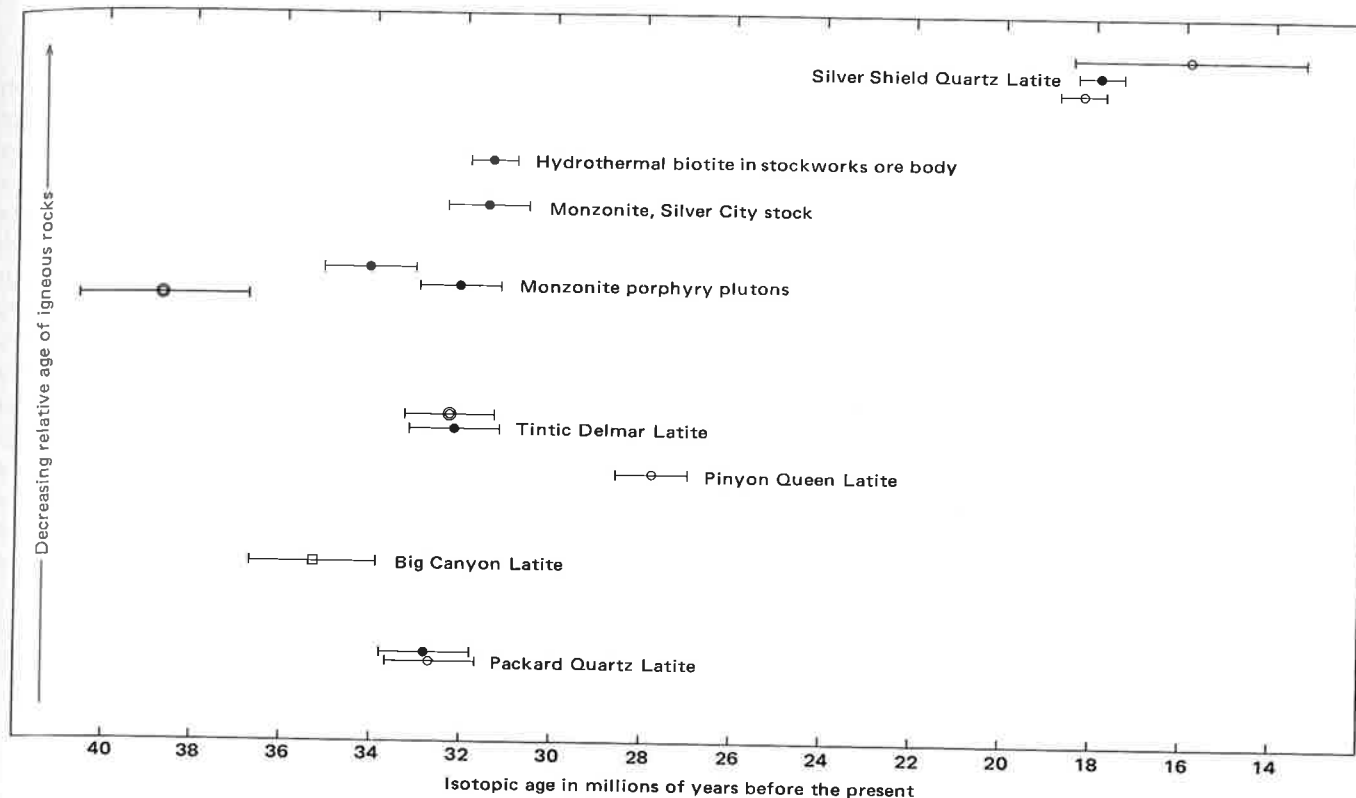
FIGURE 33. -- Summary of isotopic ages of igneous rocks of East Tintic Mountains.
