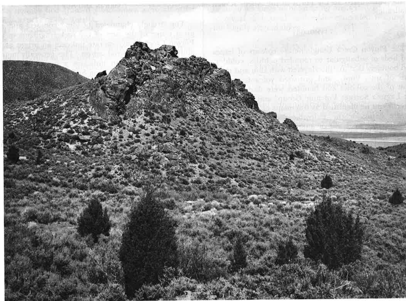
FIGURE 24. - Outcrop of Silver Shield Quartz Latite dike 1,600 ft (488 m) N. 75° W. of Silver Shield (Independence) shaft. Dike is about 135 ft (41 m) wide at the crest of ridge where it cuts Packard Quartz Latite.
