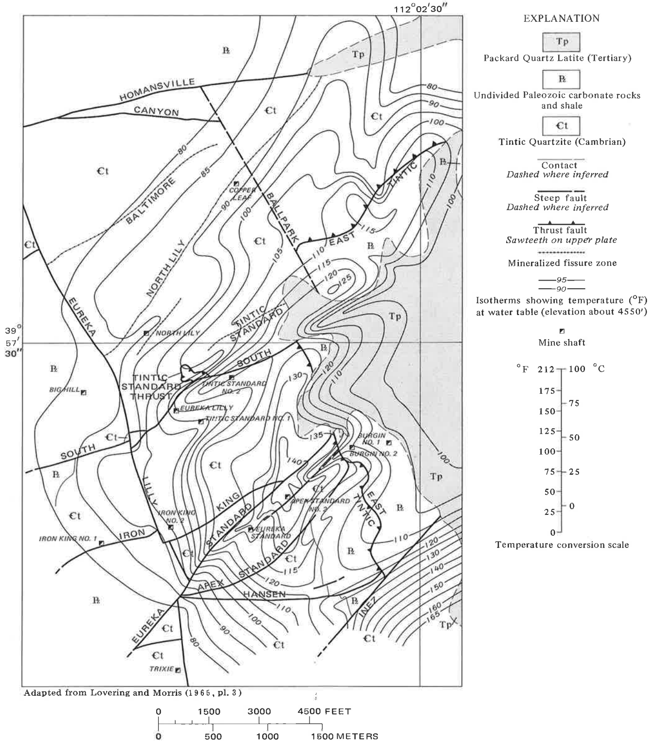
FIGURE 36. -- Simplified geologic map of East Tintic thermal area showing isotherms at elevation 4,555.
