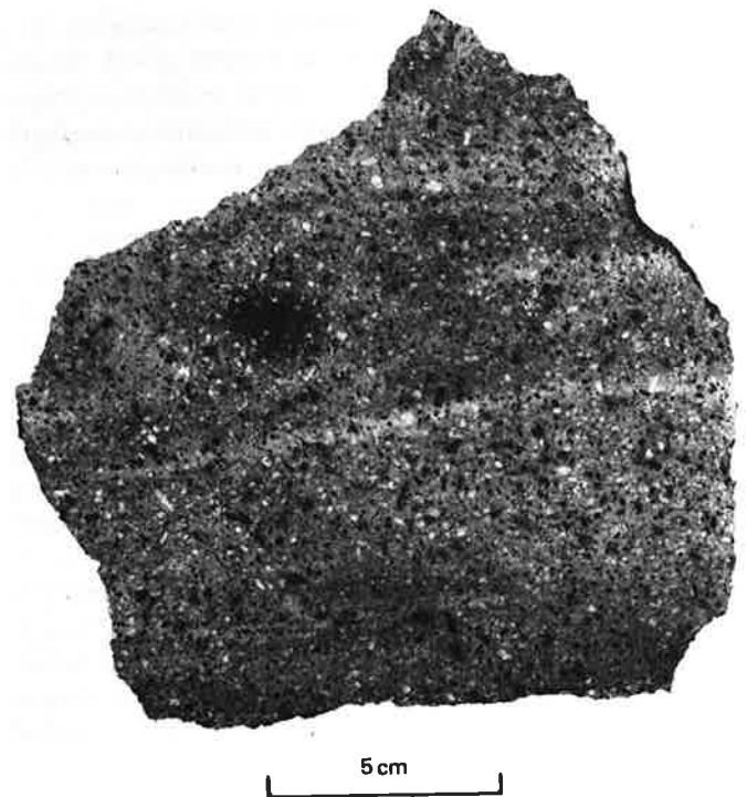
FIGURE 6. — Porphyritic unit of Packard Quartz Latite from exposure on Highway 6-50, 1,700 ft (518 m) east-southeast of Copper Leaf Shaft.
