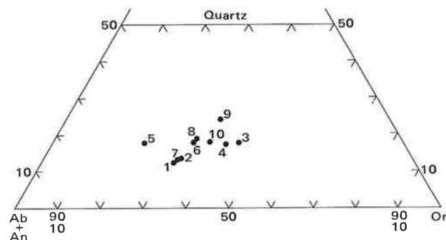
FIGURE 8. — Plot of normative quartz-orthoclase-albite ± anorthite of selected samples of the Tintic Mountain Volcanic Group and related and comparative rocks.
