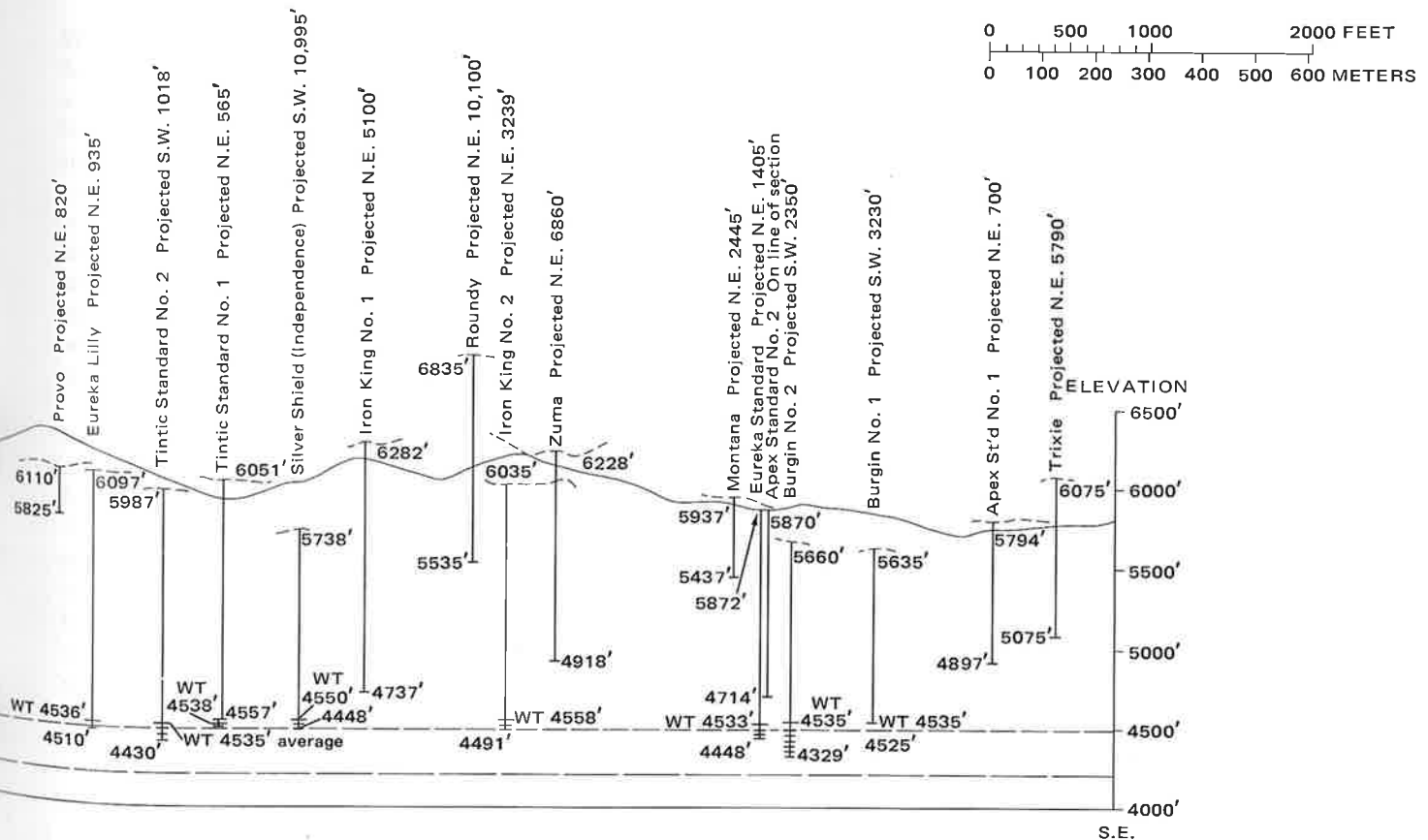
Section runs N. 40.7° W. through Apex Standard No. 2 and North Lily shafts.
