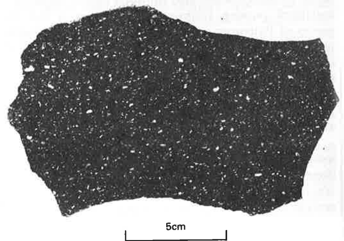
FIGURE 11. — Flow member of Big Canyon Latite from exposures on south side of entrance to Big Canyon 1 mi (1.6 km) S. 45° W. of Low Lonesome Point. Light phenocrysts are plagioclase. Same as sample 5, table 4.
