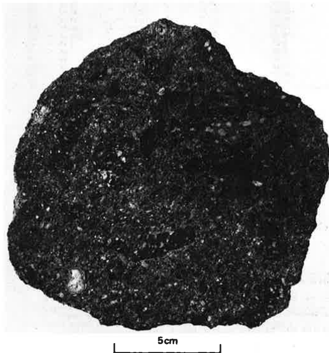
FIGURE 15. — Flow member of North Standard Latite from exposures 500 ft (152 m) due north of North Standard shaft. Dark areas are fragments of vitrophyre embedded in a vitrophyre of lighter hue.
