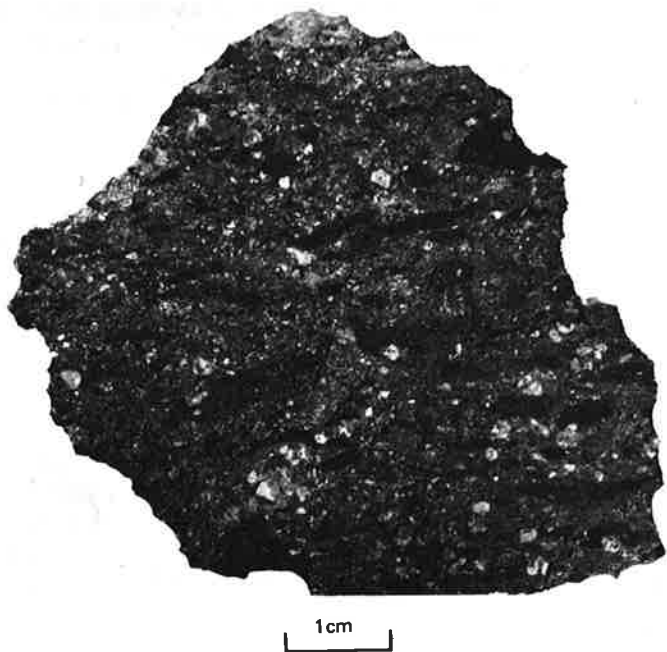
FIGURE 13. — Intrusive latite breccia from small pipe 2,500 ft (762 m) west-southwest of Low Lonesome Point. Dark areas are flattened pumice fragments; light areas are chiefly fragments of quartz latite. Same as sample 9, table 4.
