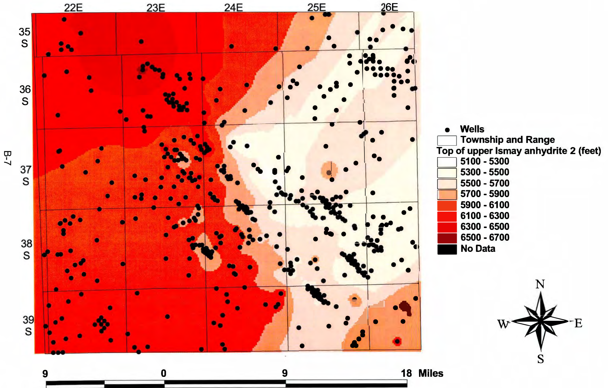
Figure B.7. Top of upper Ismay anhydrite 2, Blanding sub-basin, Utah
