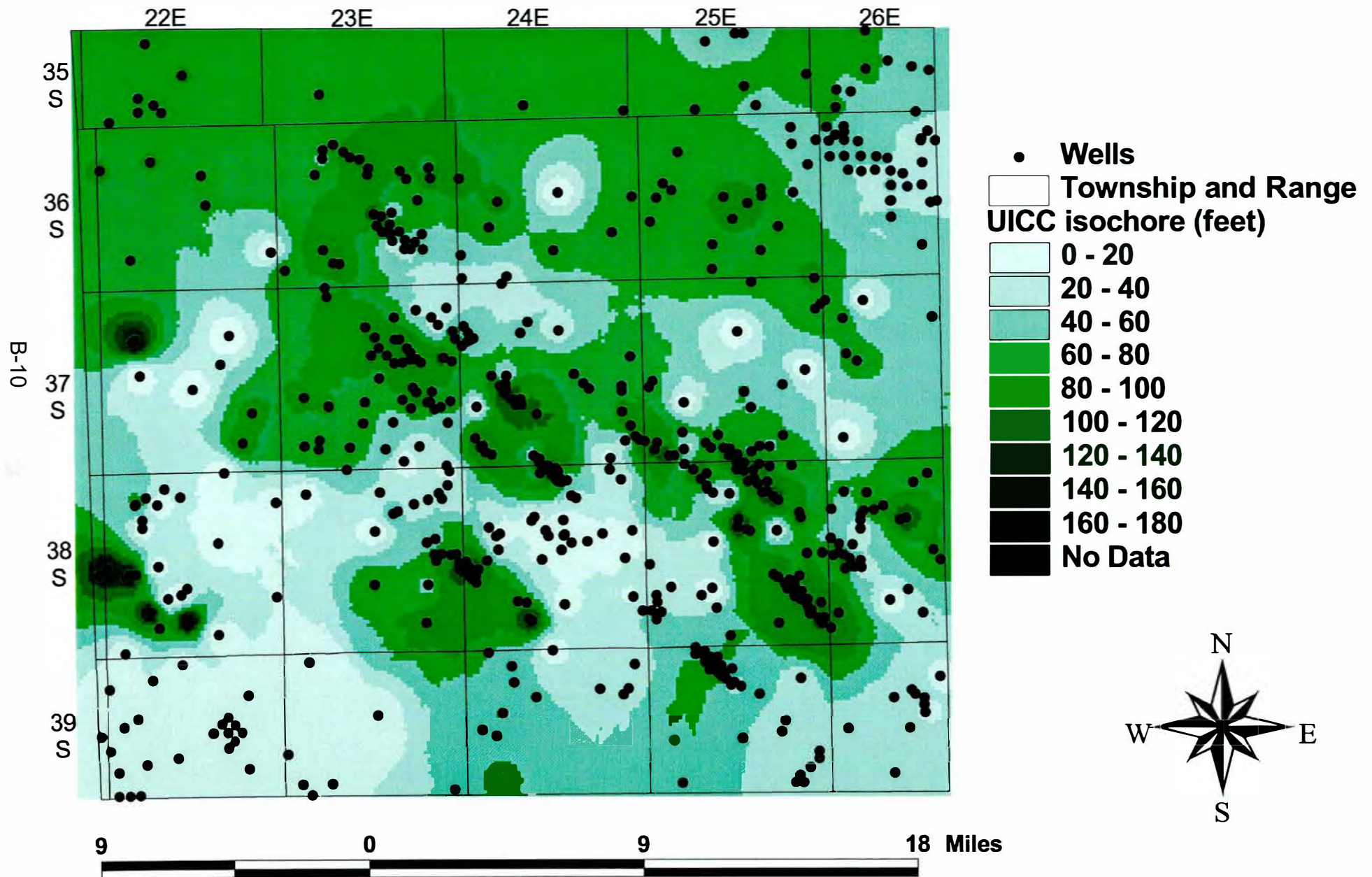
Figure B.10. Isochore of upper Ismay clean carbonate, Blanding sub-basin, Utah
