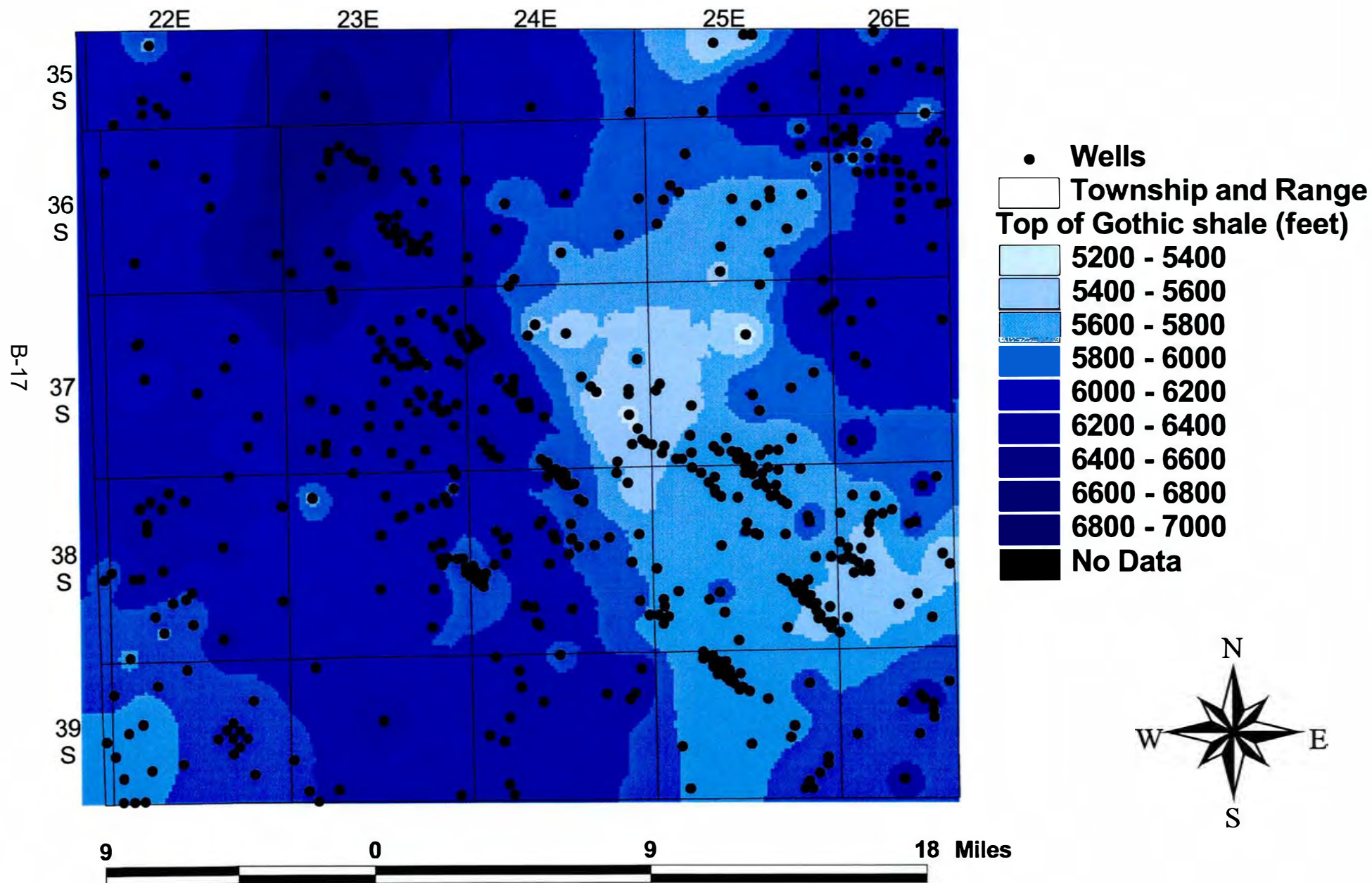
Figure B.17. Top of Gothic shale, Blanding sub-basin, Utah
