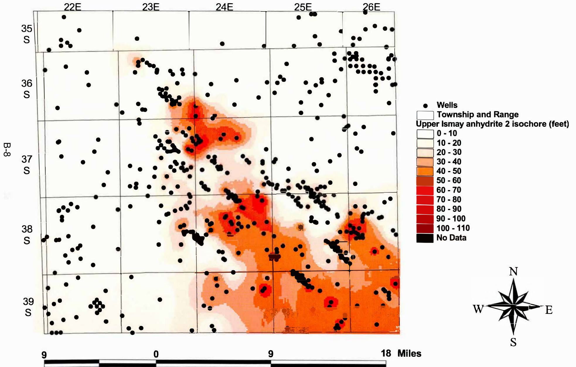
Figure B.8. Isochore of upper Ismay anhydrite 2, Blanding sub-basin, Utah
