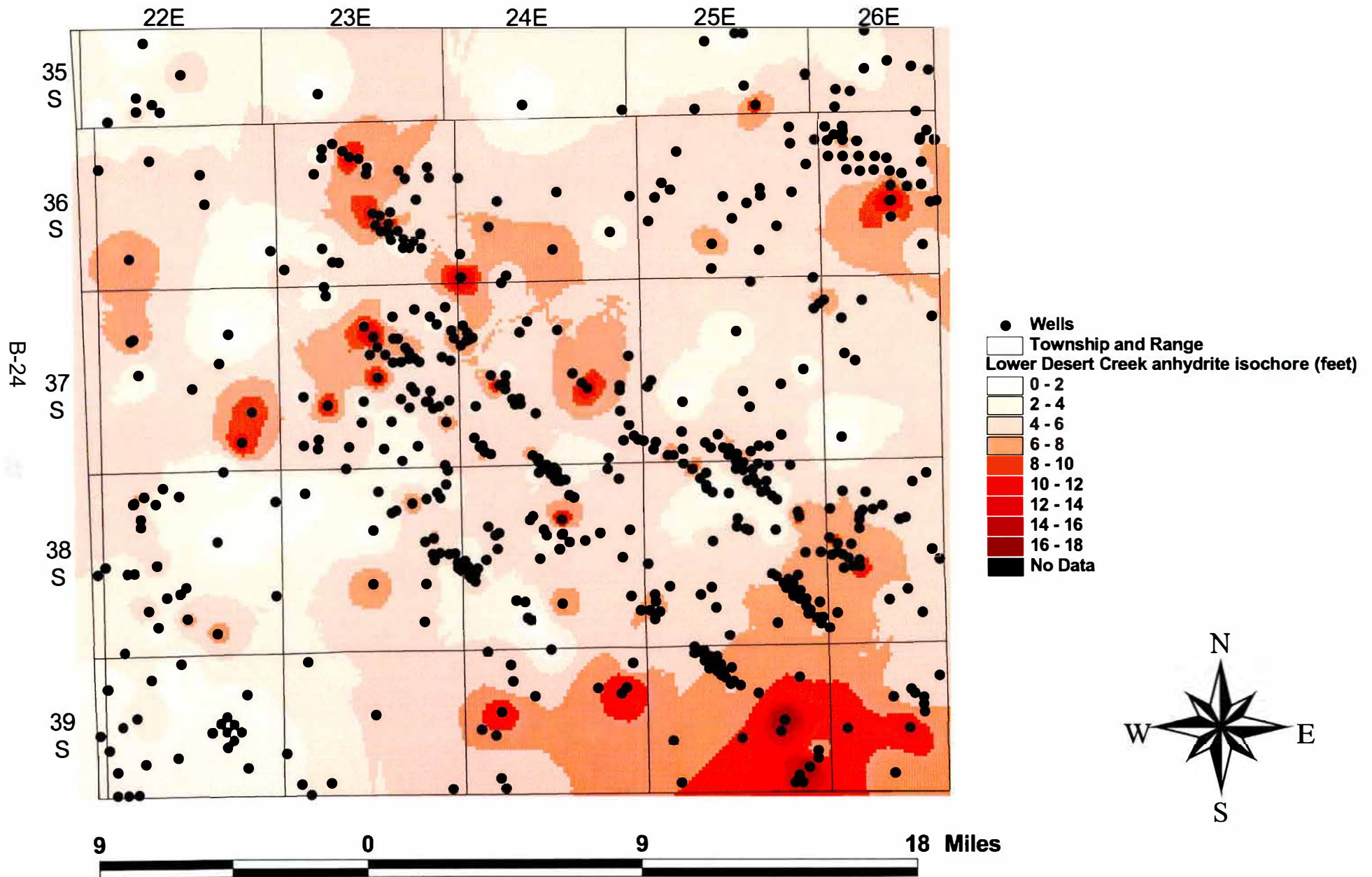
Figure B.24. Lower Desert Creek anhydrite isochore, Blanding sub-basin, Utah
