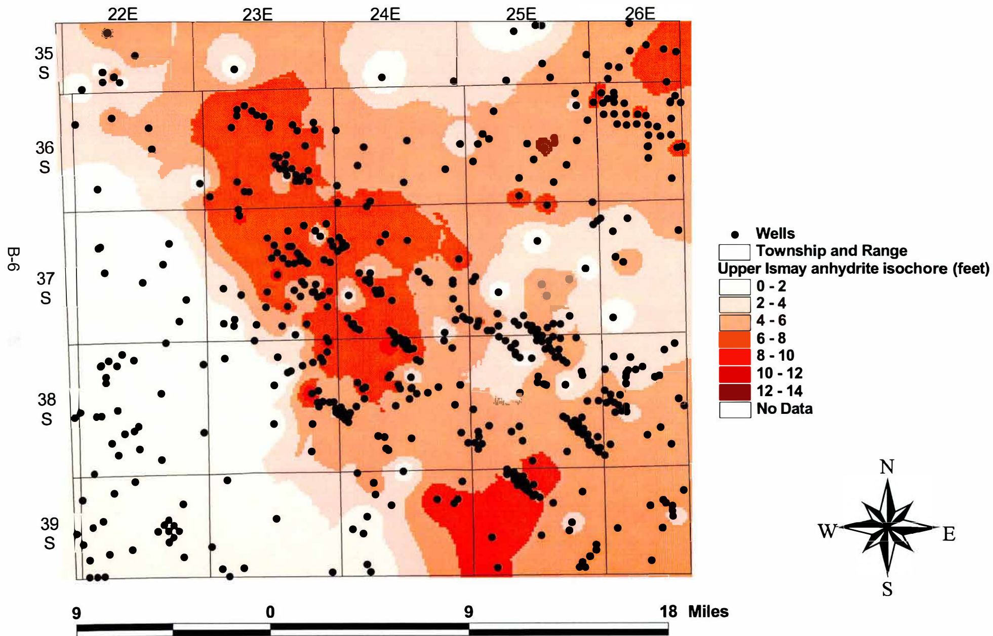
Figure B.6. Isochore of upper Ismay anhydrite, Blanding sub-basin, Utah
