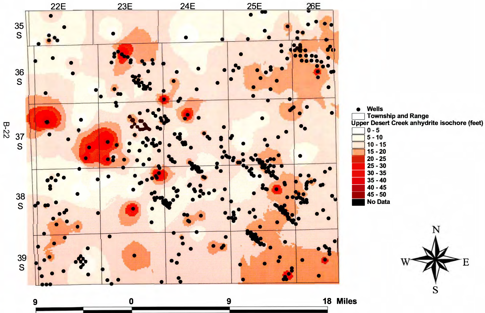
Figure B.22. Upper Desert Creek anhydrite isochore, Blanding sub-basin, Utah
