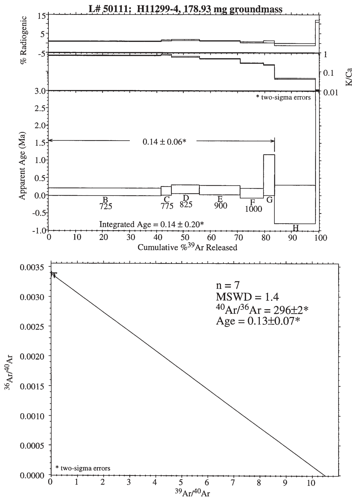
Age spectrum and isochron for H11299-4.
