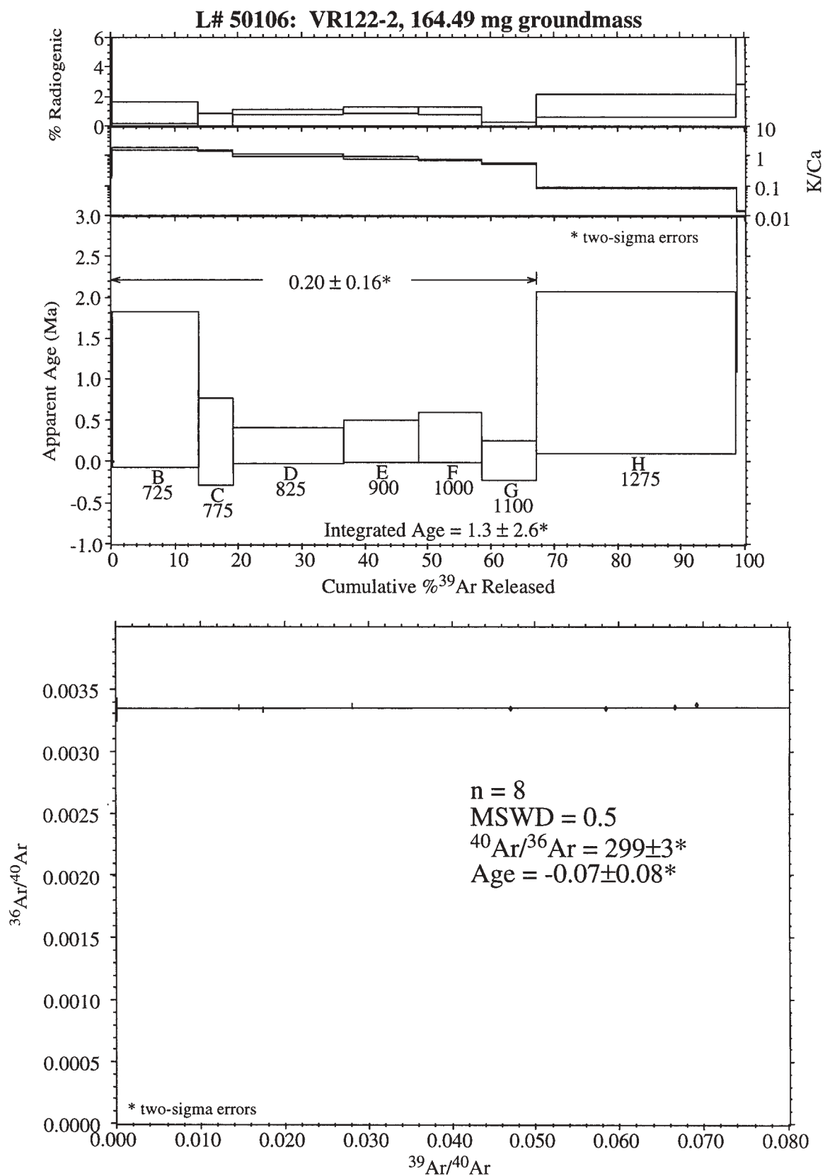
Age spectrum and isochron for VR122-2.
