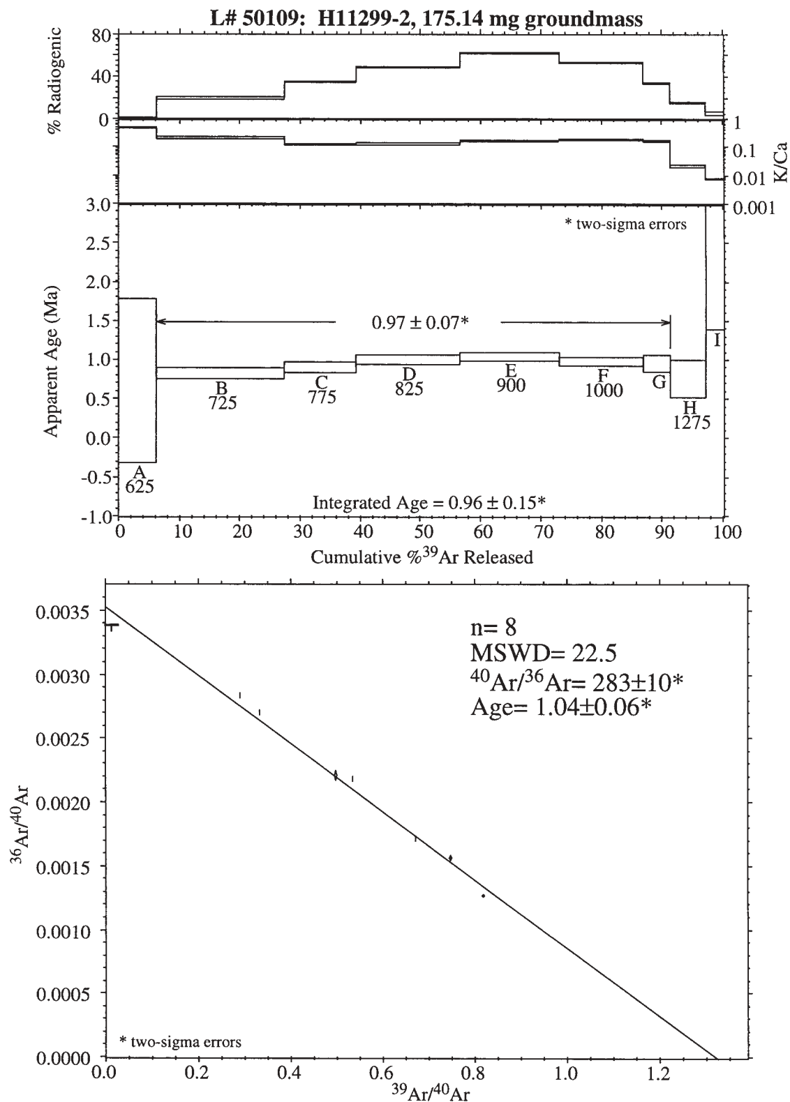
Age spectrum and isochron for H11299-2.
