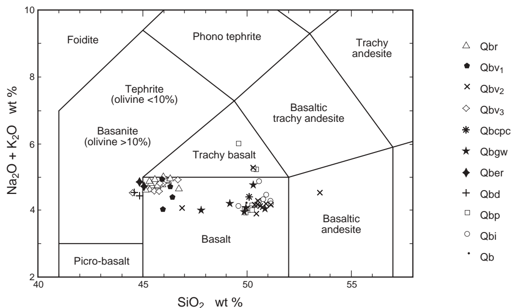
Figure 6. Geochemical classification of basalts in the Hurricane quadrangle using scheme of Le Bas and others (1986). See appendices A and B for analytical results, and figure 7 and plate 1 for sample locations. Major oxides are normalized to 100 percent. See text for explanation of map unit symbols.
