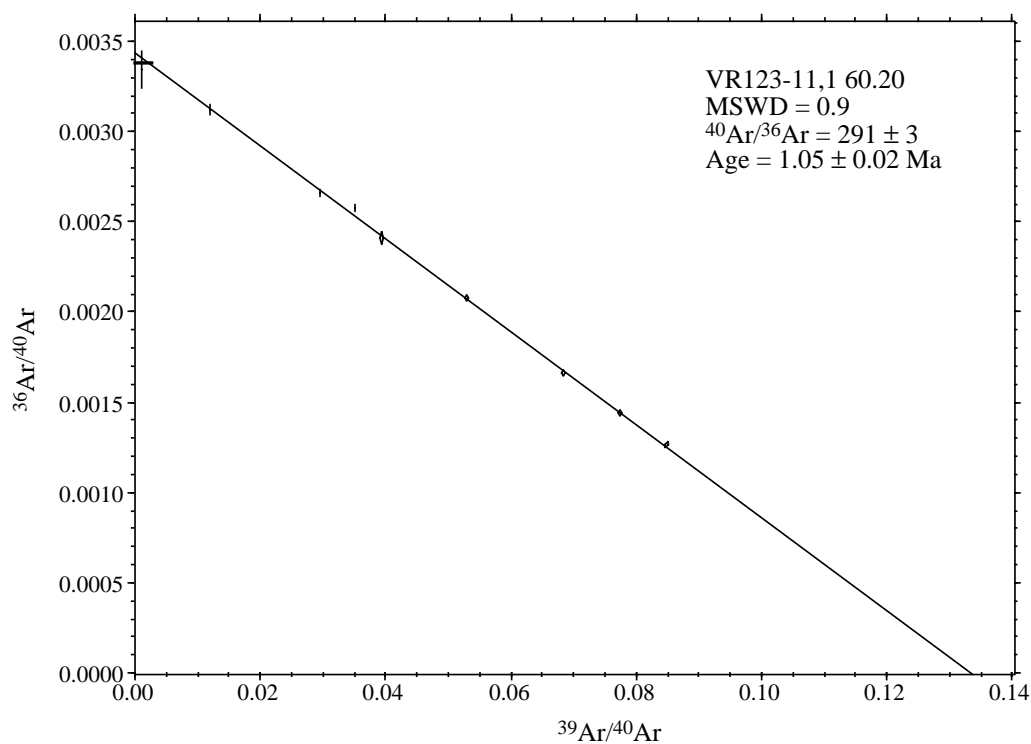
Age spectrum and isochron for VR123-11.
