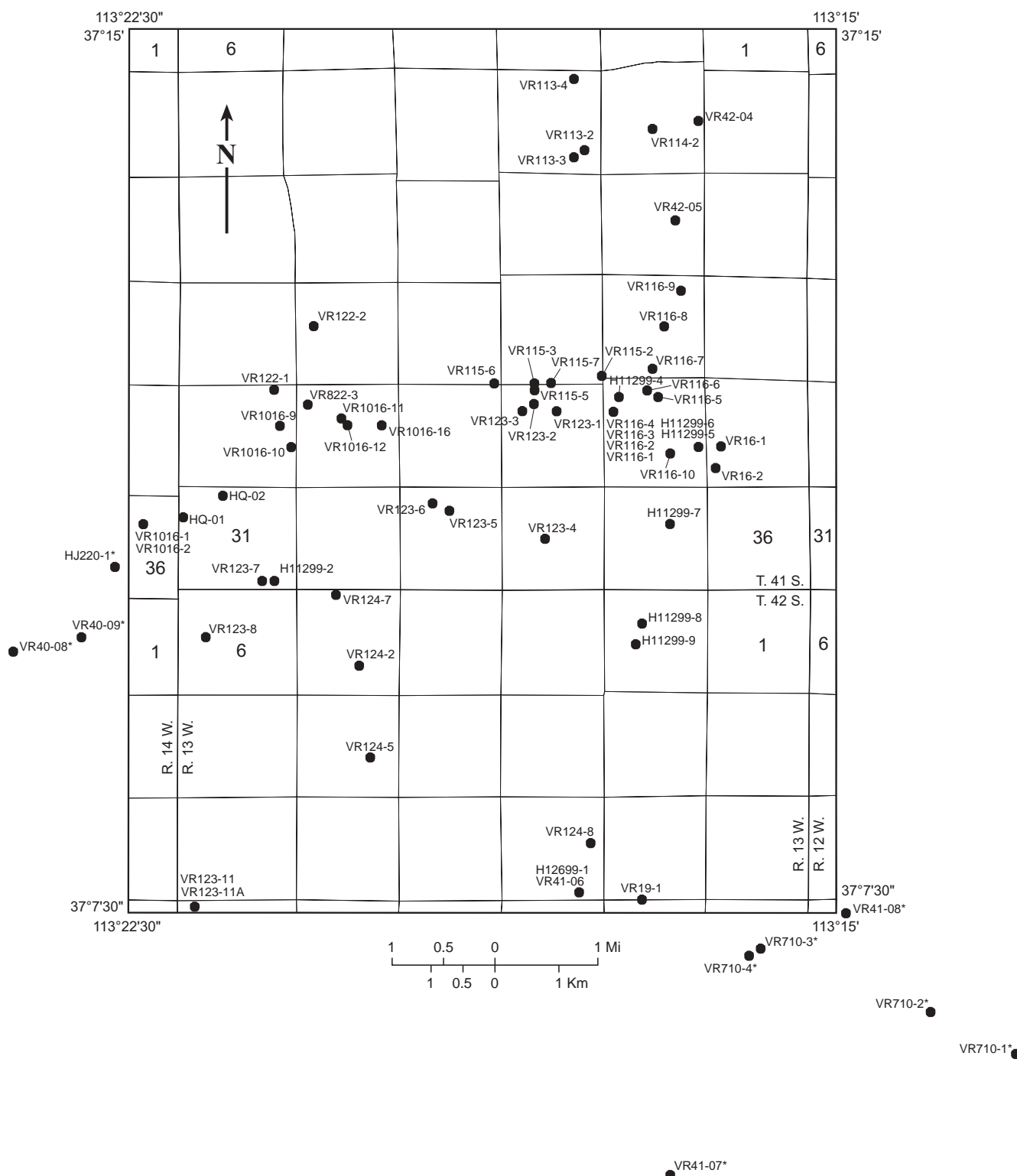
Figure 7. Basalt sample locations. For more detail, see plate 1. Asterisk indicates sample is outside the Hurricane quadrangle.
