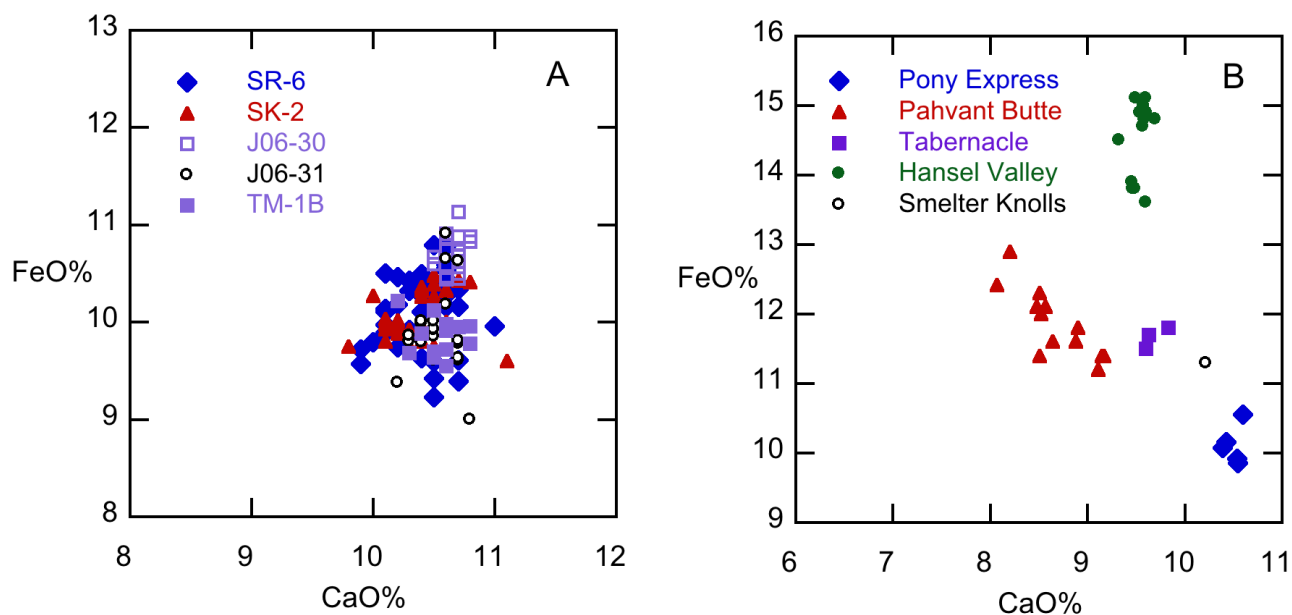
Figure 7. (A) Electron microprobe analyses of glass in individual Pony Express shards (values in weight percent iron and calcium oxides). (B) Average analyses of glass from Pony Express and regional tephras (solid symbols) and whole-rock basalts (open symbols). PBR = Pahvant Butte ridge, TH = Tabernacle Hill, SK = Smelter Knolls (Oviatt and Nash, 1989; Turley and Nash, 1980).
