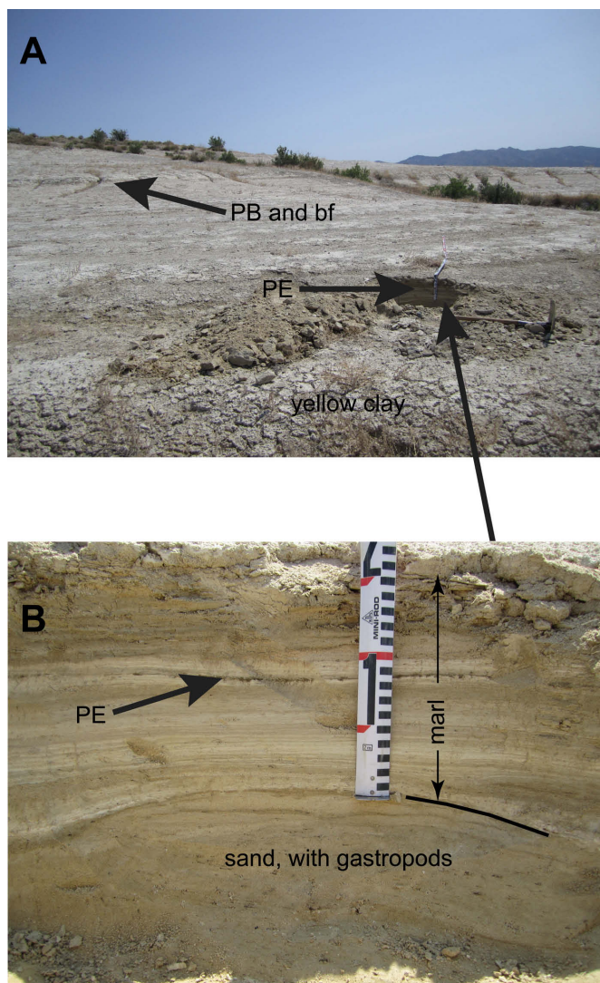
Figure 4. (A) Photograph of the Bonneville section at location TM-3 on the east bluff of the Old River Bed, directly south of the crossing of the Pony Express road. (B) Close-up view of the Pony Express ash (PE) in the Bonneville marl in the shallow pit wall shown in figure 4A. The scale, numbered in decimeters, starts at the base of the Bonneville marl. PB = Pahvant Butte basaltic ash; bf = Bonneville flood marker horizon in the marl, about 2 cm higher than PB. (Photos by Oviatt, 2012.)
