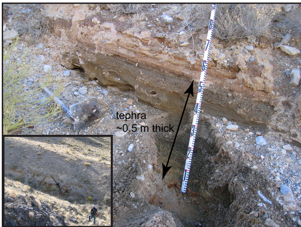
Figure 6. Photograph of the exposure of tephra exposed in a gully at locality J06-30 on the east flank of Camels Back Ridge on Dugway Proving Ground. (Photos by Donald Clark [UGS], 2006).
