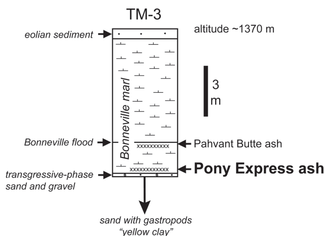
Figure 3. Measured section of Lake Bonneville deposits at locality TM-3, on the east bluff of the Old River Bed, just south of the point where it is crossed by the Pony Express road (table 1; figure 2). Both the Pony Express ash and the Pahvant Butte basaltic ash are present in this section. For further information on this section, see Gilbert (1890), Oviatt (1987), and Oviatt and others (1994a, 1994b). Core TM-5 (Oviatt and others, 1994a) was taken at locality TM-3.
