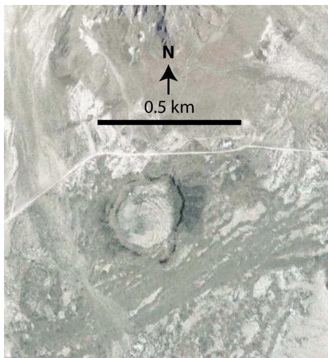
Figure 5. Satellite image of the Smelter Knolls maar, western Sevier Desert (112.853° W; 39.403° N), a possible source vent for the Pony Express ash. The maar was produced by an eruption through an older basalt flow. Note the Lake Bonneville marl deposits (white) and beach gravels (dark) that overlie the basalt flow. Image from Google Earth (2012).
