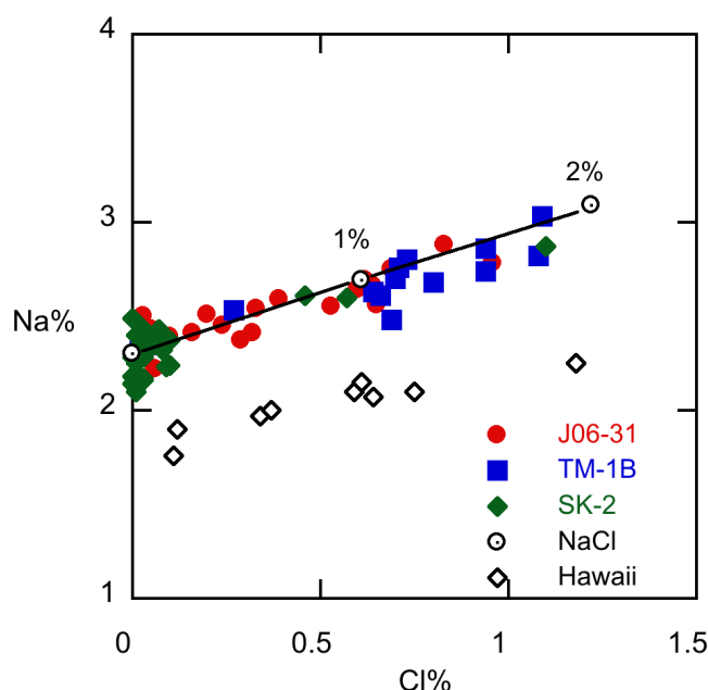
Figure 8. Electron microprobe analyses of Cl in Pony Express glass (values in weight percent). Solid line represents mixing between low-Cl Pony Express glass and NaCl. Hawaii basalt data for comparison are from Coombs and others (2004).
