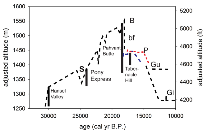
Figure 1. Schematic diagram showing changes in lake level in Lake Bonneville (dashed line) and approximate ages and altitude limits of the four well-documented basaltic ashes in Lake Bonneville sediments. Lake-level chronology based on Oviatt and others (1992), Oviatt (1997), Godsey and others (2011), Miller and others (2012), and Reheis and others (in review). S = Stansbury shoreline zone; B = Bonneville shoreline; P = Provo shoreline; Gu = Gunnison shoreline (Sevier Desert basin); Gi = Gilbert shoreline (Great Salt Lake basin); bf = Bonneville flood. The two alternatives for Provo-shoreline chronology (short red-dashed line and blue long-dashed line) are from Miller and others (2012). Altitudes adjusted for the effects of differential isostatic rebound using the Curry equation (Oviatt and others, 1992). Ages are given in calibrated years before present. The basaltic ashes in the Bonneville basin (except for the Sevier Lake ash, which is not well dated and is only found at one locality) are shown by black lines that show the altitudinal limits of known outcrops of each ash.
