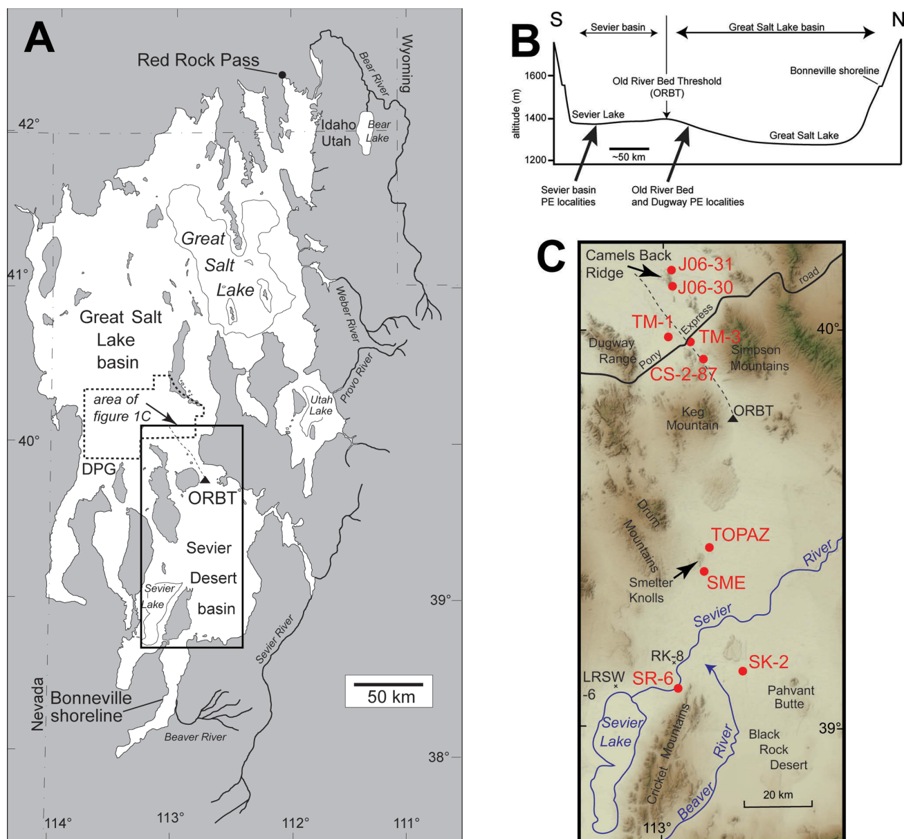
Figure 2. (A) Map of the maximum extent of Lake Bonneville in western Utah, eastern Nevada, and southern Idaho. ORBT = Old River Bed threshold, the topographic divide between the Sevier Desert and Great Salt Lake basins; fine dashed line is the Old River Bed. Red Rock Pass is the post-flood overflow point of Lake Bonneville at the Provo shoreline. DPG = Dugway Proving Ground, boundary marked as dotted line. (B) Schematic north-south topographic profile across the Sevier Desert basin and the Great Salt Lake basin, showing the shallow Sevier Desert basin and the ORBT. (C) Enlarged shaded-relief map of part of map 2A showing localities where Pony Express ash has been found; see table 1 for location coordinates. Localities LRSW-6 and RK-8 are mentioned in the text. Fine dashed line is the Old River Bed.
