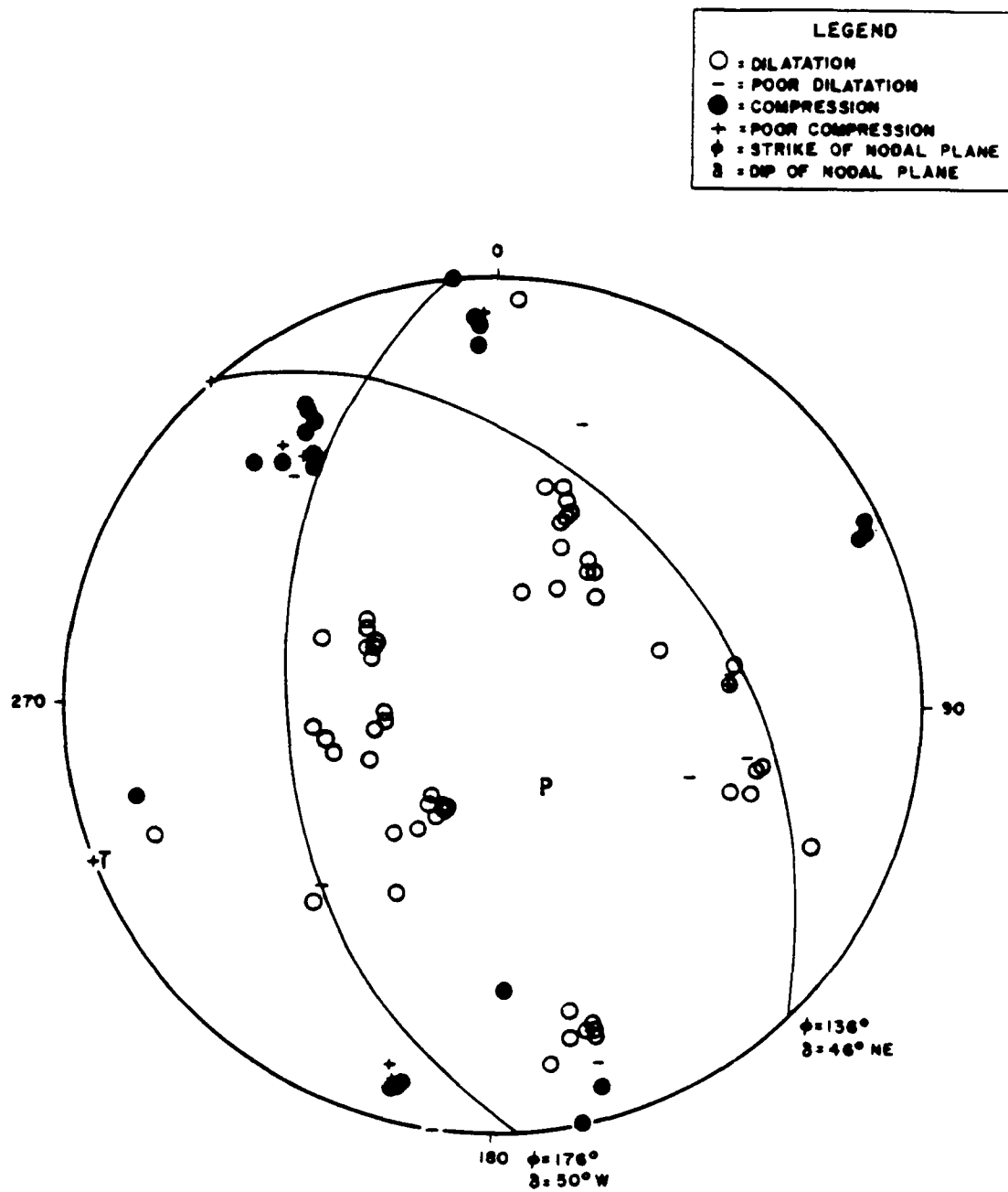
Figure 4.1. Composite focal mechanism solution No. 1 for 1980 Bear Wallow earthquakes No. 58-63, 73, 74, 79-87. First motion polarities plotted on lower hemisphere, equal area projection. P and T indicate compressional and tensional axes, respectively.
