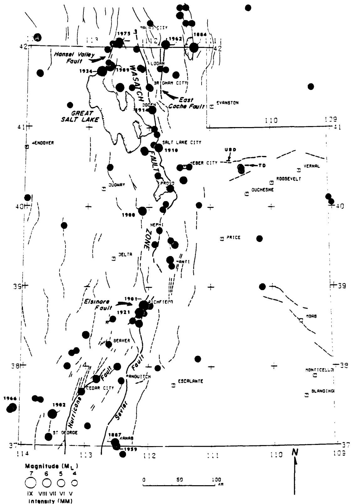
Figure 3.5. Epicenter map of the largest historical earthquakes in the Utah region, 1850-1978. For coincident epicenters, only the largest event is shown. Earthquakes of magnitude 5.5 or greater are dated by year. Cenozoic faults shown for reference. Taskeech and Upper Stillwater damsites are indicated by TD and USD, respectively (modified from Arabasz and Smith, 1979).
