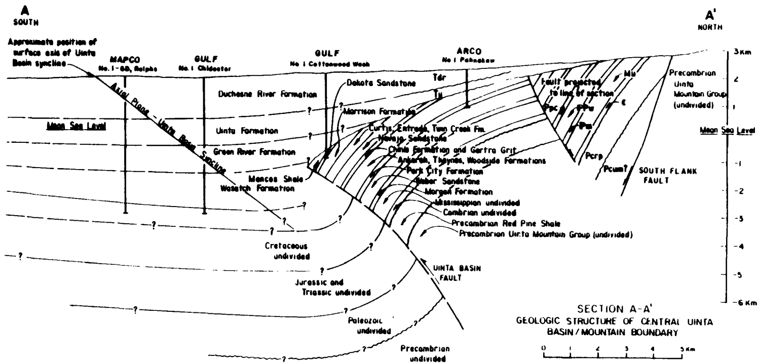
Figure 3.3. Geologic cross section (A-A'; fig. 3.2) of the south flank of the Uinta Mountains and northern Uinta Basin (modified from Campbell, 1975).
