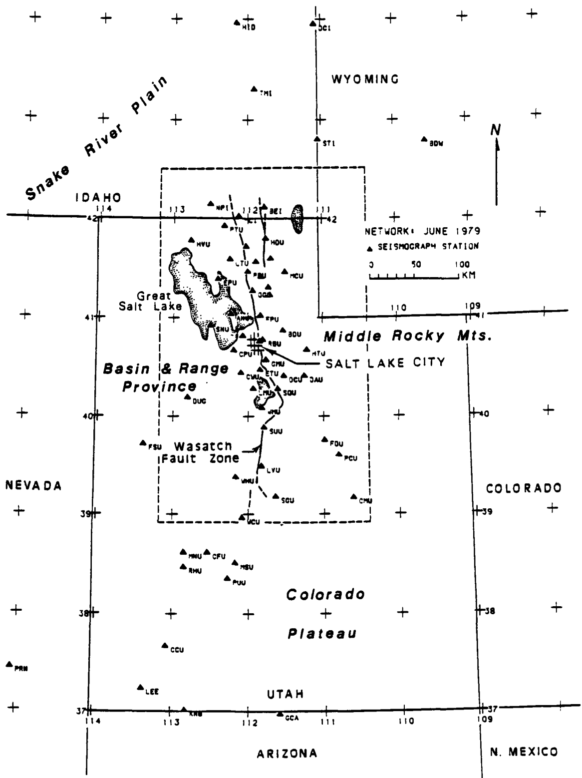
Figure 3.6. Location map of the University of Utah telemetered seismic network as of June 1979. Dashed line outlines area illustrated in figure 3.7 (Arabasz and others, 1979).
