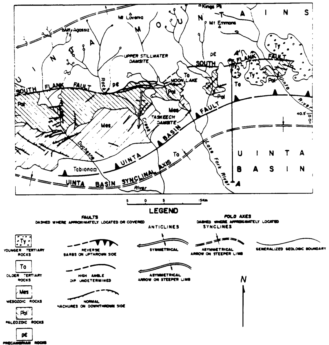
Figure 3.2. Generalized geologic map of the Uinta Mountains and Uinta Basin in the vicinity of Taskeech and Upper Stillwater damsites (modified from Campbell, 1975).
