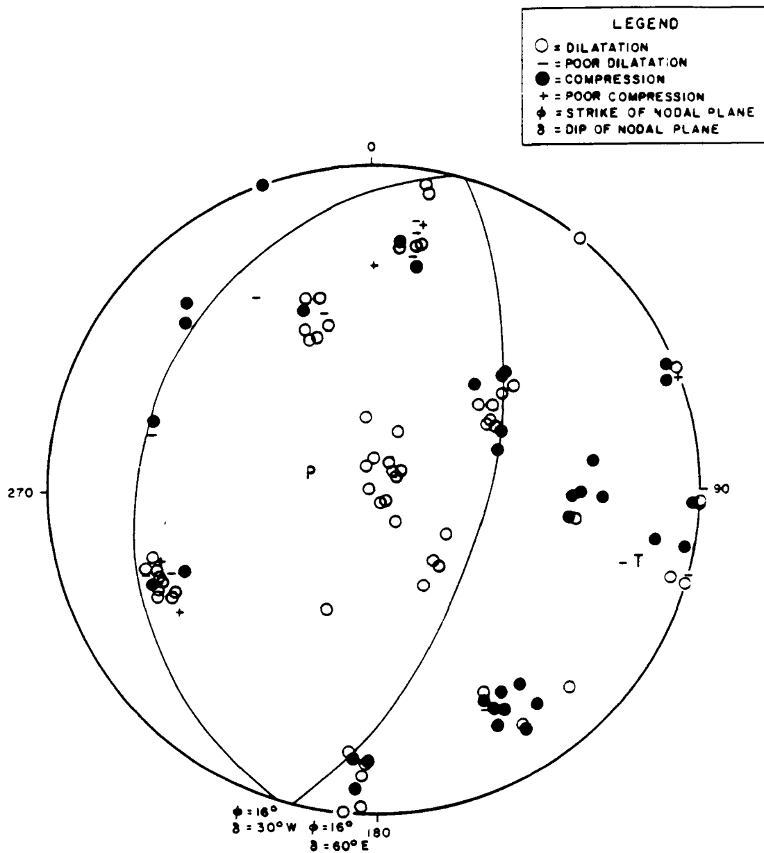
Figure 4.3. Composite focal mechanism solution for Bear Wallow earthquakes No. 15, 21, 24, 42, 48, 49, 51, 53, 55, 57, 64, 66, 71, 75, 76, and 77. First motion polarities plotted on lower hemisphere, equal area projection. P and T indicate compressional and tensional axes, respectively.
