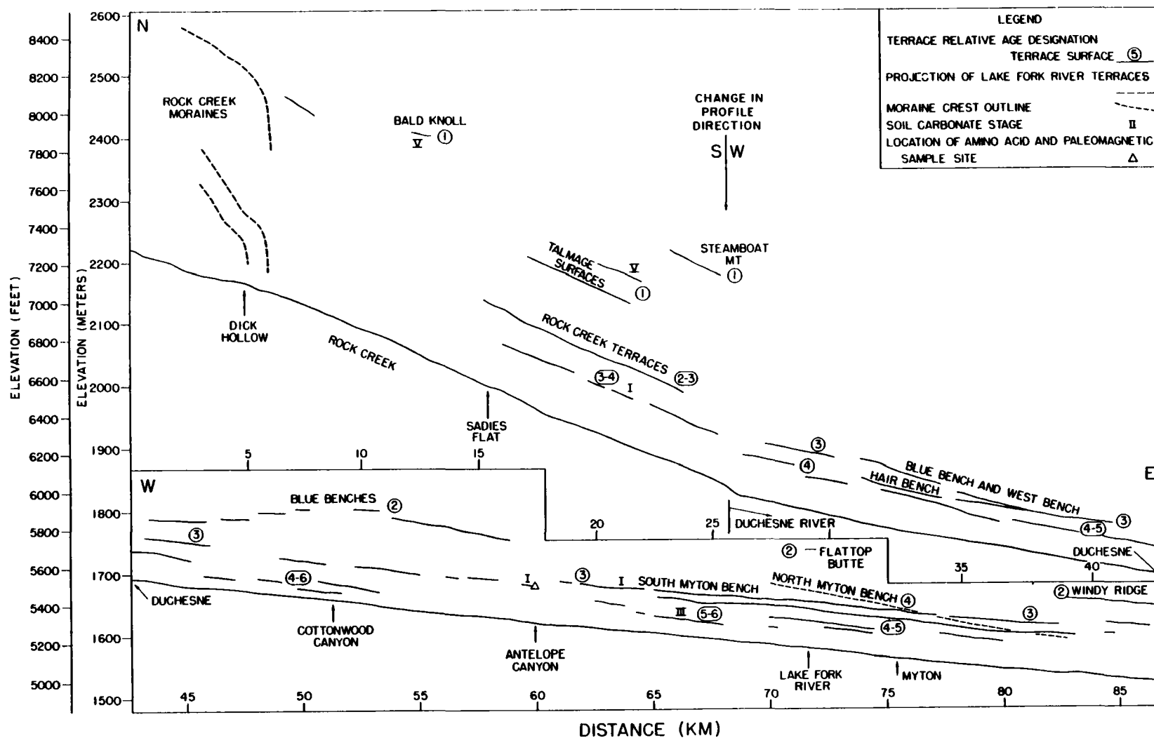
Figure A.2. Terrace surface profiles along Rock Creek and Duchesne River showing the projection of correlative surfaces along the Lake Fork River, moraine crest outlines, soil carbonate stage (Gile and others, 1966) in exposures, and the location of the Antelope Canyon gravel pit where paleomagnetic and amino acid samples were collected. Terrace surfaces have been numbered using the relative-age groups defined using the terraces along the Lake Fork River (fig. A.1).
