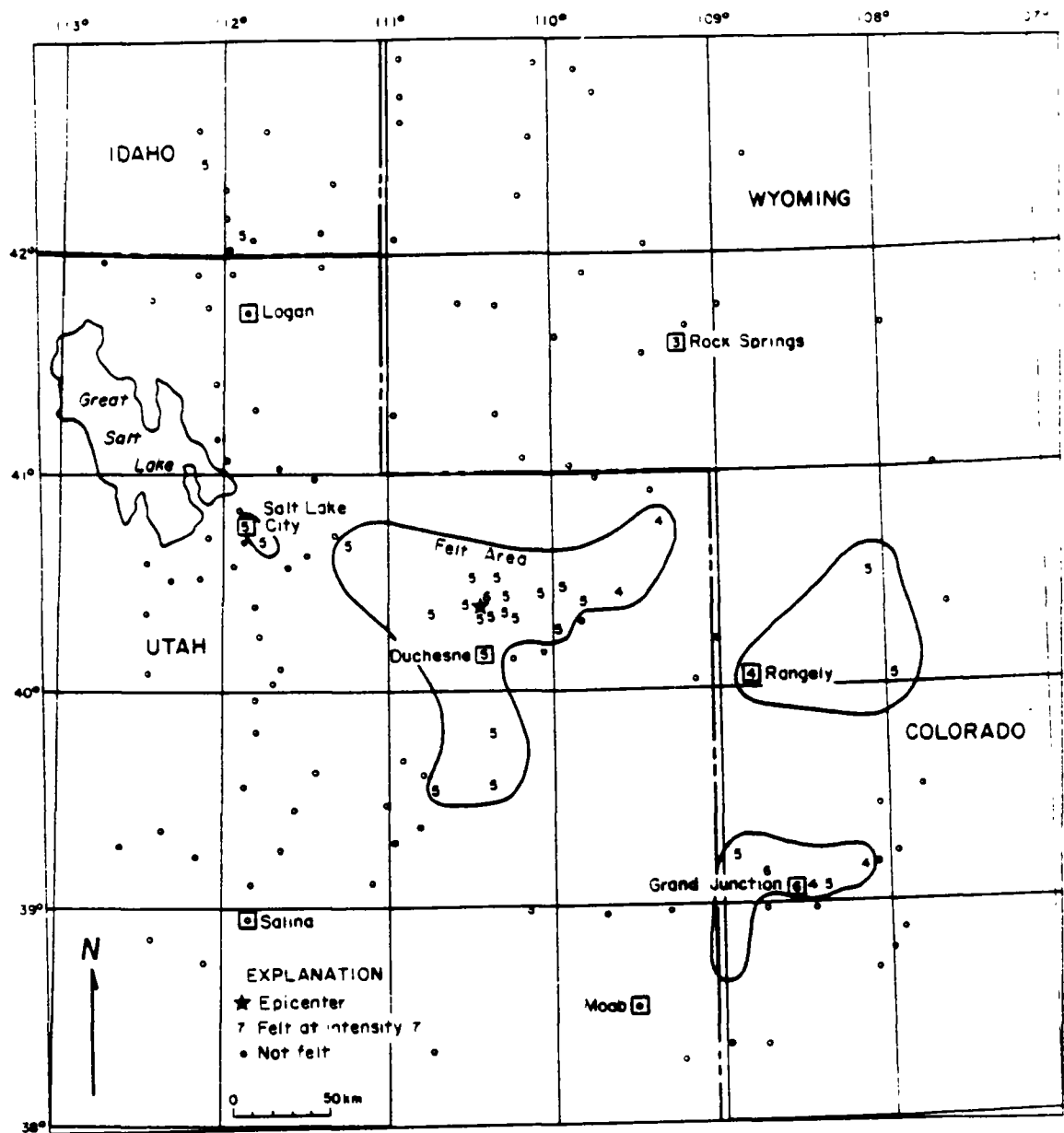
Figure 3.9. Isoseismal map of the September 30, 1977 magnitude 4.5 earthquake near Moon Lake, Utah. Arabic numerals represent reported Modified Mercalli intensities (from USGS, 1977).
