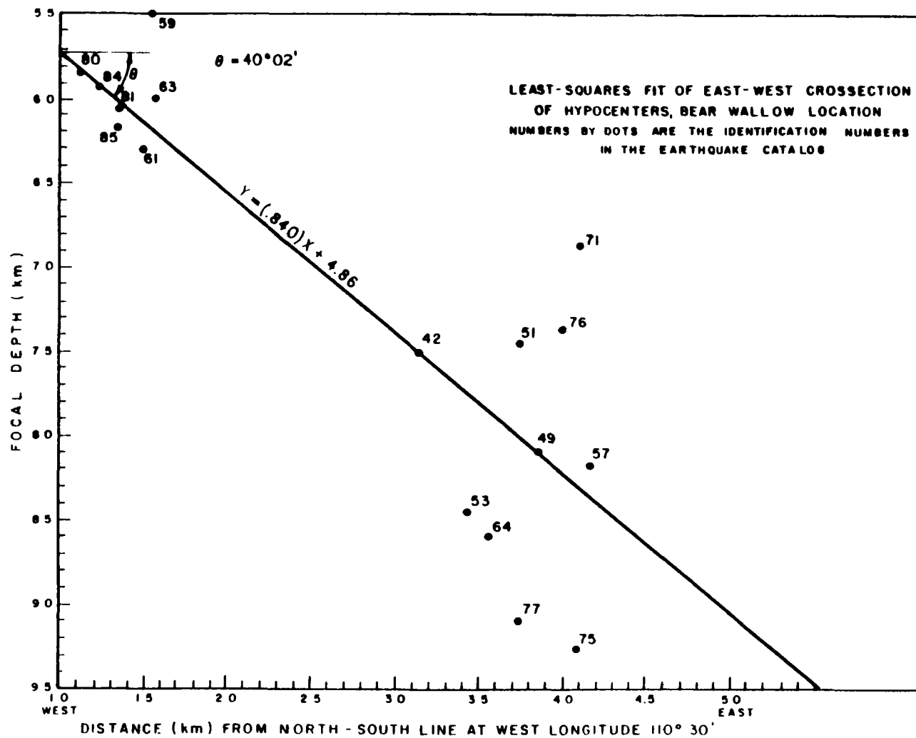
Figure 4.4. East-west hypocentral cross section (A-A') of selected Bear Wallow events.
