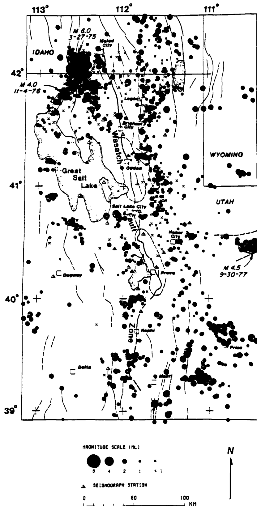
Figure 3.7. Epicenter map of the Wasatch Front earthquakes, October 1974 to June 1978. Seismic gaps along the Wasatch fault are outlined by dashed lines. Cenozoic faults shown for reference (from Arabasz and others, 1979).
