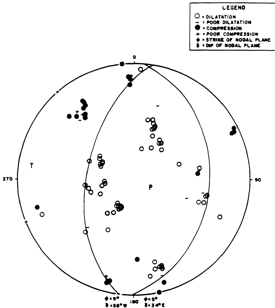
Figure 4.2. Composite focal mechanism solution No. 2 for 1980 Bear Wallow earthquakes No. 58-63, 73, 74, 79-87. First motion polarities plotted on lower hemisphere, equal area projection. P and T indicate compressional and tensional axes, respectively.
