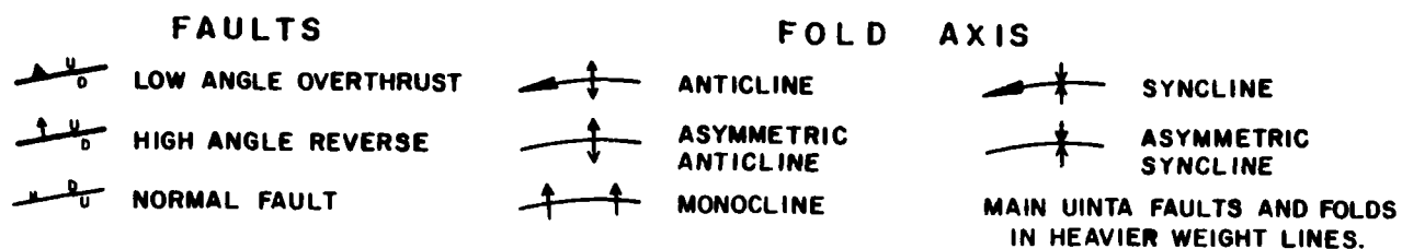
Figure 3.4. Generalized tectonic map of the Uinta Mountains (modified from Ritzma, 1969).
