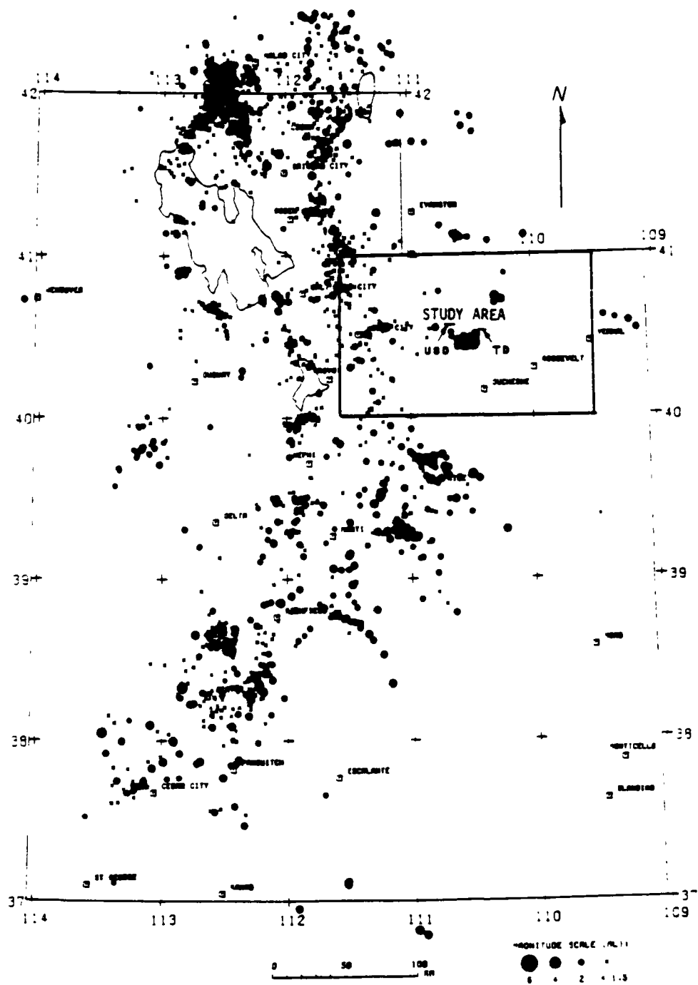
Figure 3.8. Study area location map and Utah earthquakes, October 1974 to June 1978. Taskeech and Upper Stillwater damsites are indicated by TD and USD, respectively (modified from Richins, 1979).
