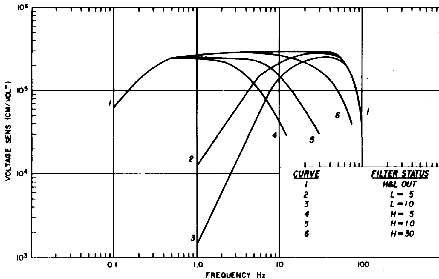
Figure D.1. Typical voltage sensitivity at maximum gain for the MEQ 800 amplifier/recorder.
