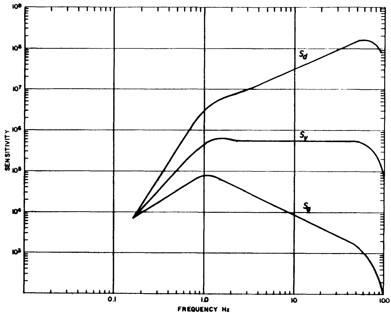
Figure D.3. Maximum sensitivity for the MEQ 800/L-4C seismograph system. Displacement - S_d cm/cm, Velocity - S_v cm/cm/sec, Acceleration - S_a cm/cm/sec 2 .
