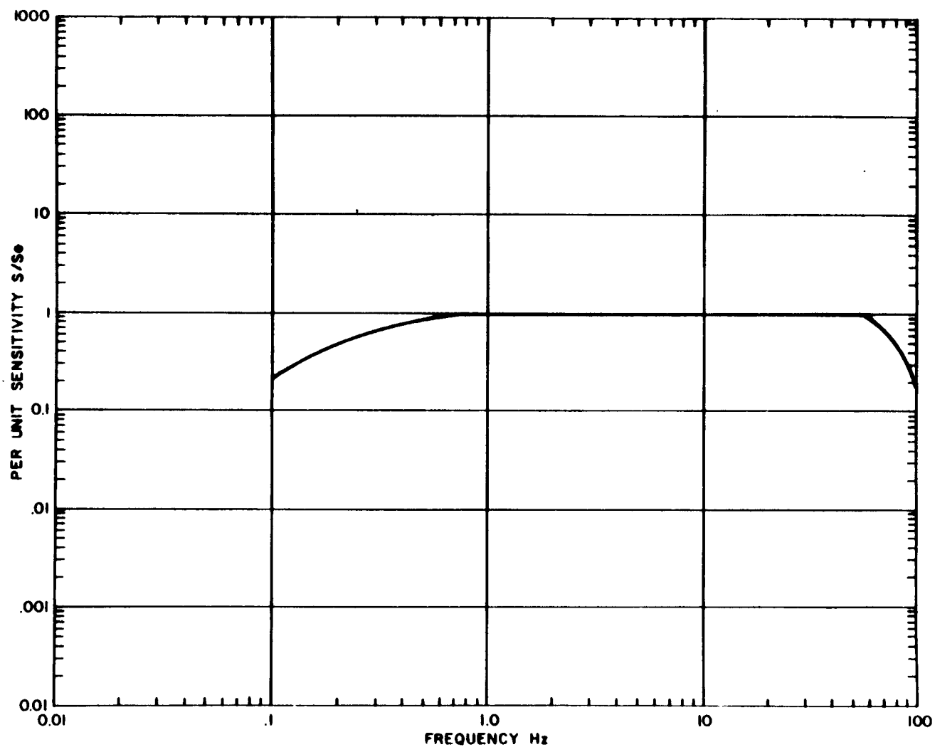
Figure D.2. Voltage response characteristics for the MEQ 800 amplifier/recorder (normalized to unity, both filters "OUT").
