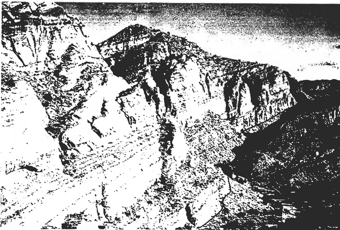
Figure 5 Looking north at the transition zone of the basal Navajo Sandstone; photo taken from the Red Cliffs Recreation Area overlook, NENE 1/4 section 15, T.41S., R.14W. Note planar bedded strata and thin, slope-forming mudstone intervals in lower part of transition zone. The contact with the underlying Kayenta Formation (shown) is at the base of the lowest cliff-forming sandstone; the hill on the right is capped by Navajo Sandstone.
