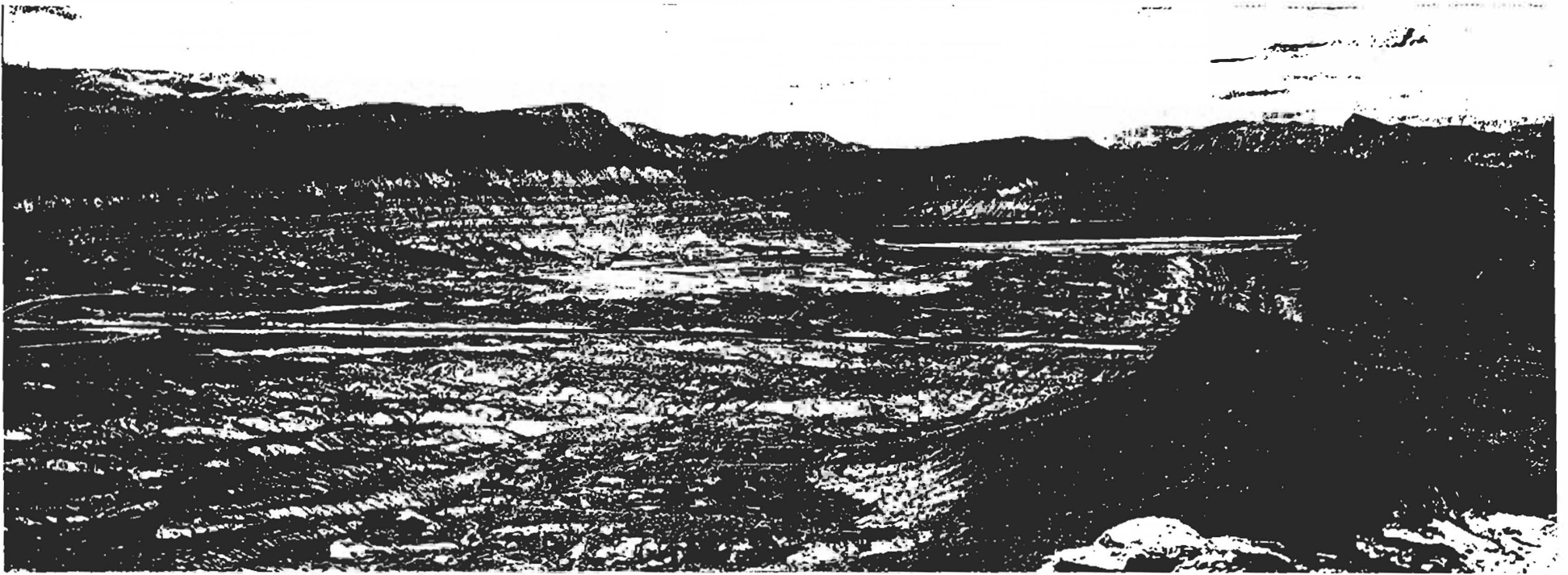
Figure 4 Looking northeast toward Quail Creek reservoir, along the axis of the Virgin anticline; photo taken from the SE 1/4 section 3, T.42S., R.14W. Resistant Shinarump Conglomerate strata form the flanks and crest of the anticline, below which are ledgy slopes of the upper red member of the Moenkopi Formation. The light band near the base of the upper red member is informally known as the "Purgatory Sandstone." Red-and-white banded strata of the Shnabkaib Member forms the eroded floor of the anticline. Note bright white beds below Quail Creek dike, which were scoured clean from the catastrophic dike failure of January 1, 1989. Note also the deeply dissected landslide deposit north of Quail Creek reservoir. State Highway 9 cuts across center of photograph.
