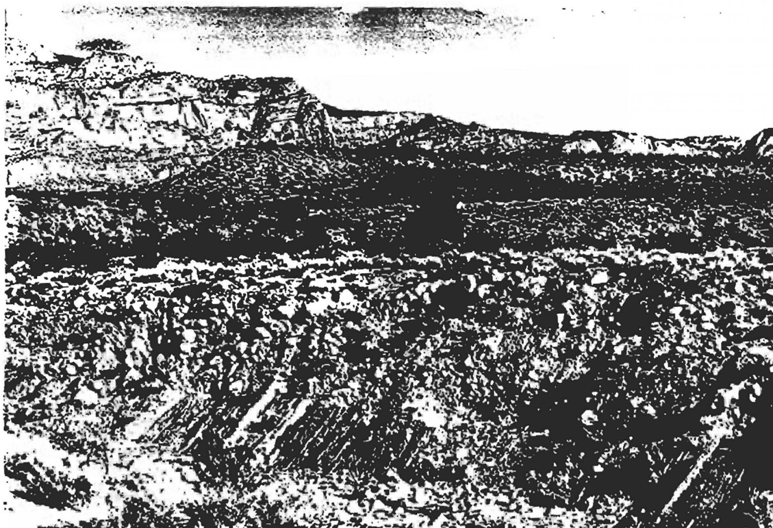
Figure 8 Looking north across Cottonwood Creek at terrace gravels overlying steeply dipping Kayenta strata; photo taken from the SENW 1/4 section 27, T.41S., R.14W. Terrace deposits in the foreground are mapped as Qal 3 , those in the middle distance, beyond the small tree, as Qal 4 , while the highest terrace level is mapped as Qao 5 . The Navajo Sandstone forms cliffs in the background.
