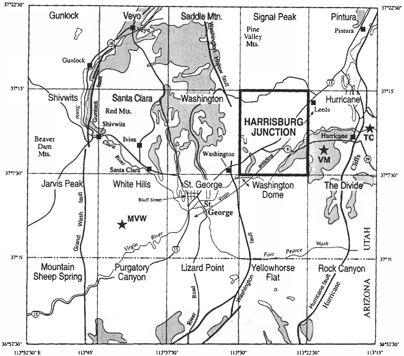
Figure 1 Location of the Harrisburg Junction and surrounding quadrangles, with major geographic and geologic features; basalt flows are shaded. This quadrangle is one of several 7.5' quadrangles recently mapped as part of the UGS effort to map the rapidly growing St. George basin. Additional geologic maps and reports are available for the Santa Clara quadrangle (Willis and Higgins, 1996), St. George quadrangle (Higgins and Willis, 1995), Washington quadrangle (Willis and Higgins, 1995), and the White Hills quadrangle (Higgins, 1997). The Hurricane and Washington Dome quadrangles are scheduled for completion in 1998. VM = Volcano Mountain and Ivan's Knoll; MVW = Mountain Valley Wash; TC = Timpoweap Canyon.
