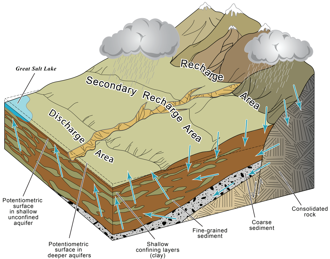
Figure 2. Generalized block diagram showing water-bearing formations, probable direction of ground-water movement (arrows), and areas of recharge and discharge, Salt Lake Valley, Salt Lake County, Utah (modified from Hely and others, 1971, Thiros and Manning, 2004).
