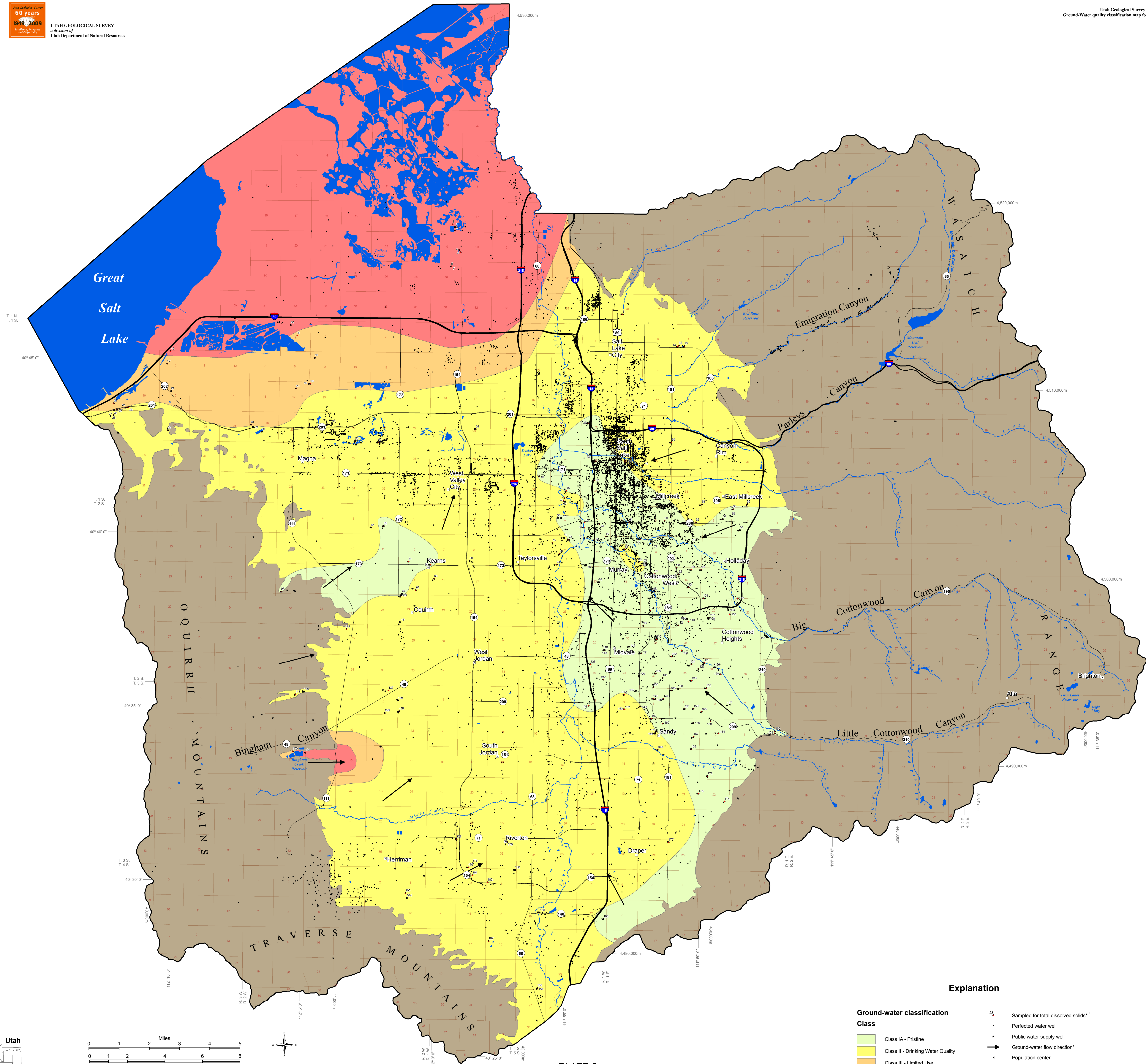
PLATE 2 GROUND-WATER QUALITY CLASSIFICATION MAP FOR THE BASIN-FILL AQUIFER, SALT LAKE VALLEY, SALT LAKE COUNTY, UTAH by Janae Wallace and Mike Lowe
