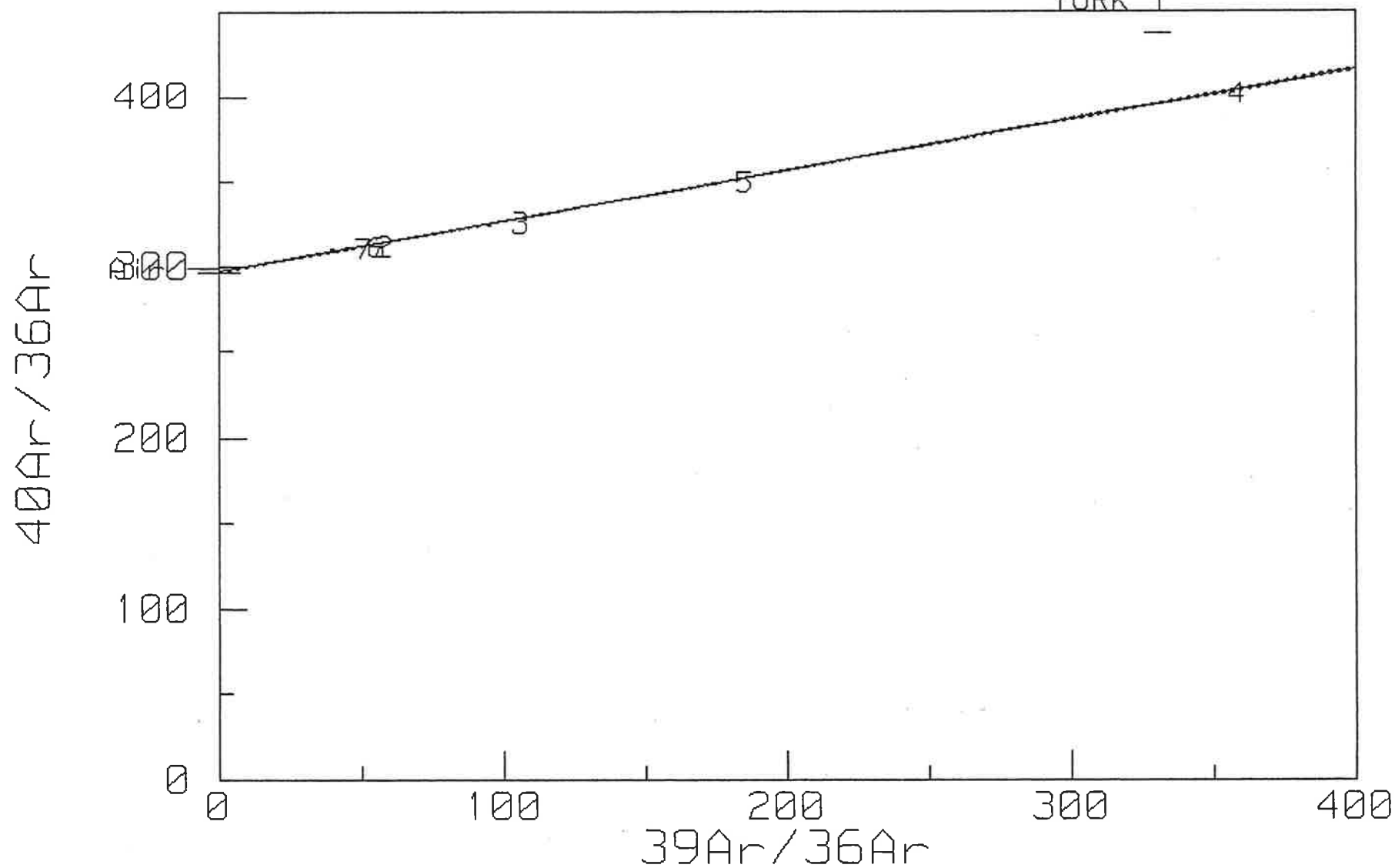
VR42-09/83+84 Ar Isochron YORK 1
