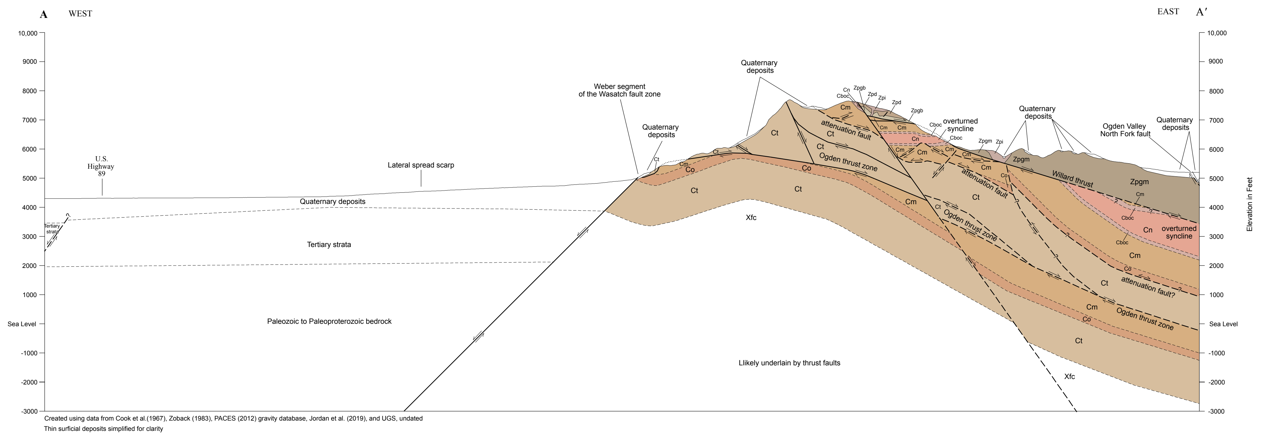
Created using data from Cook et al. (1967), Zoback (1983), PACES (2012) gravity database, Jordan et al. (2019), and UGS, undated Thin surficial deposits simplified for clarity
