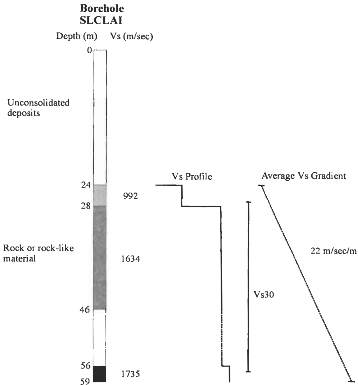
Figure 1. Schematic diagram showing interval in borehole SLCLAI with rock or rock-like material. Rock Vs30 was calculated over a 30-meter-thick interval overlapping the three distinct rock-like layers. Average gradient was determined over the entire interval of rock-like material. Borehole SLCLAI data from Tinsley and others (1991) except between 46 and 56 meters (dashed part of Vs profile) where Vs profile of Adan and Rollins (1993) used.
