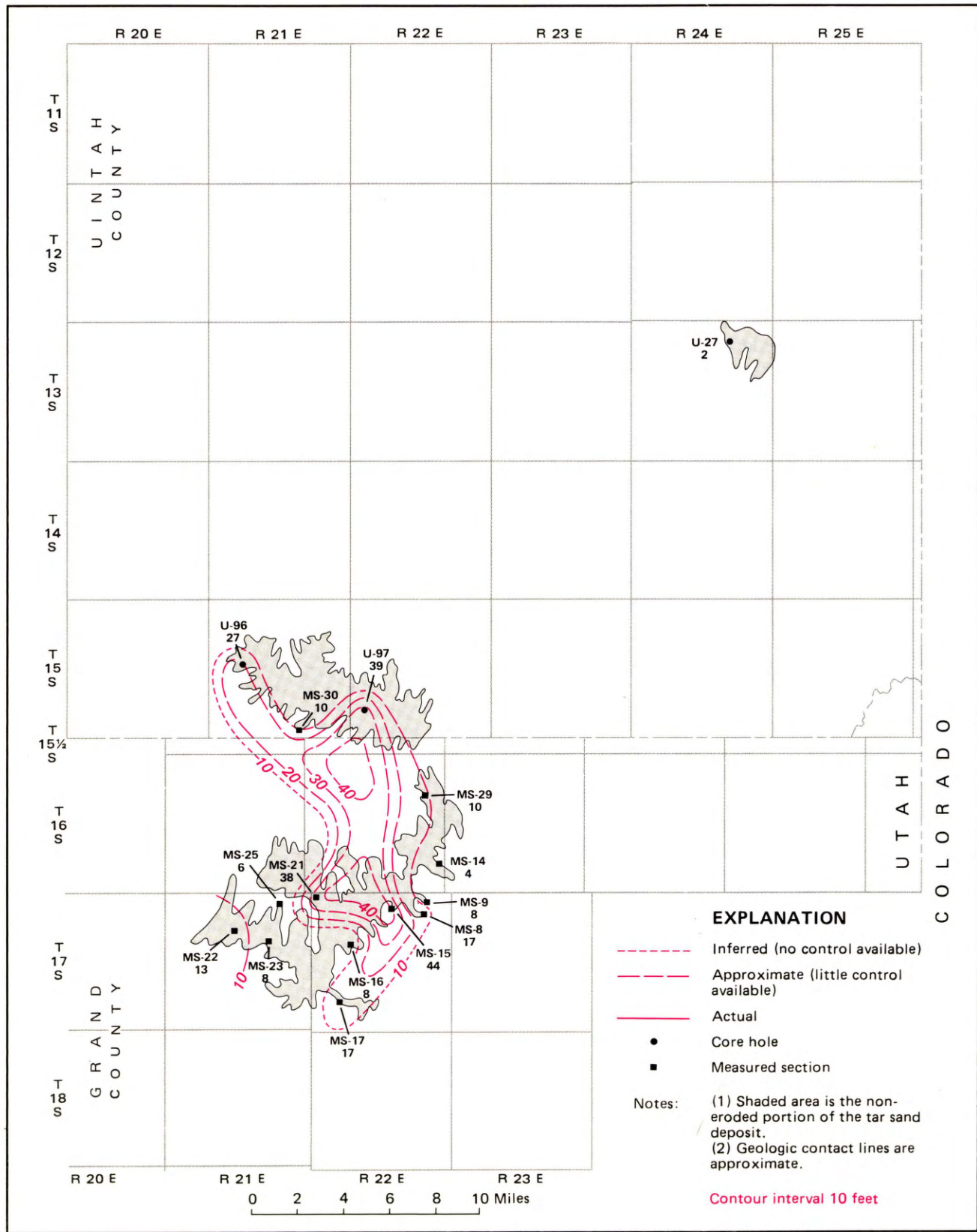
FIGURE 16. Isopach map of visibly saturated tar sand in Zone "E".
