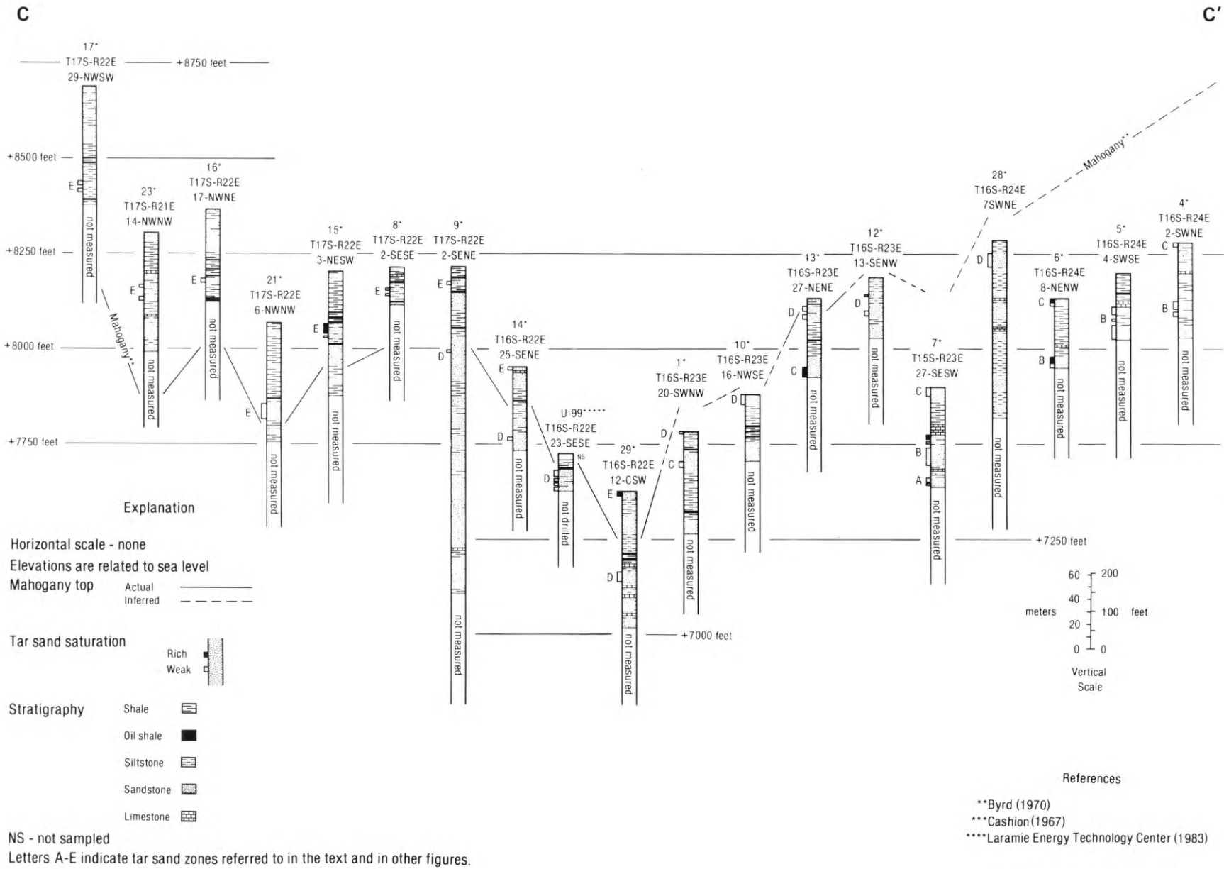
FIGURE 6. Section C-C' — Correlation of measured sections and drill holes to top of Mahogany oil shale and to tar sand zones (see figure 3).
