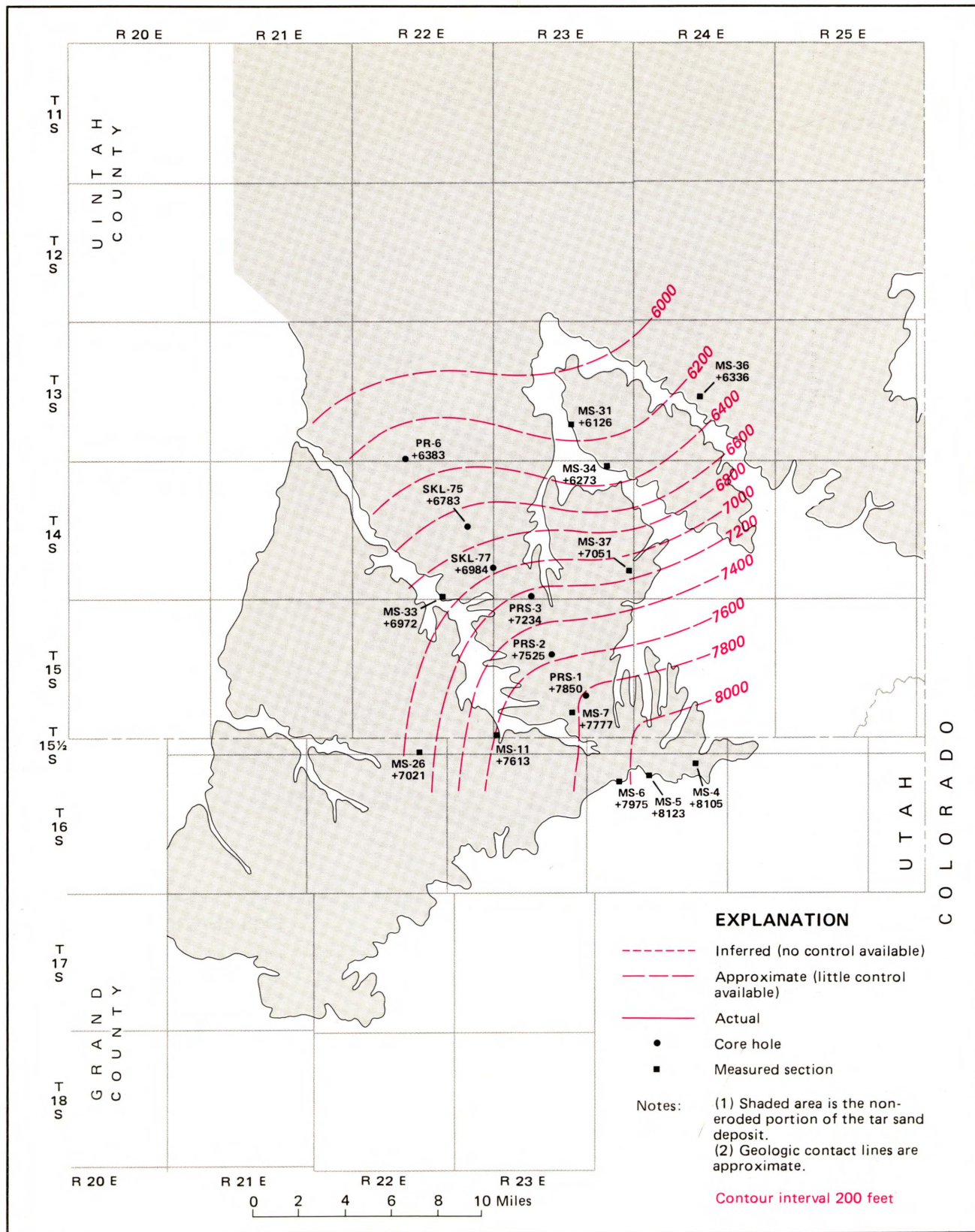
FIGURE 8. Structure contour map on top of Zone "B".
