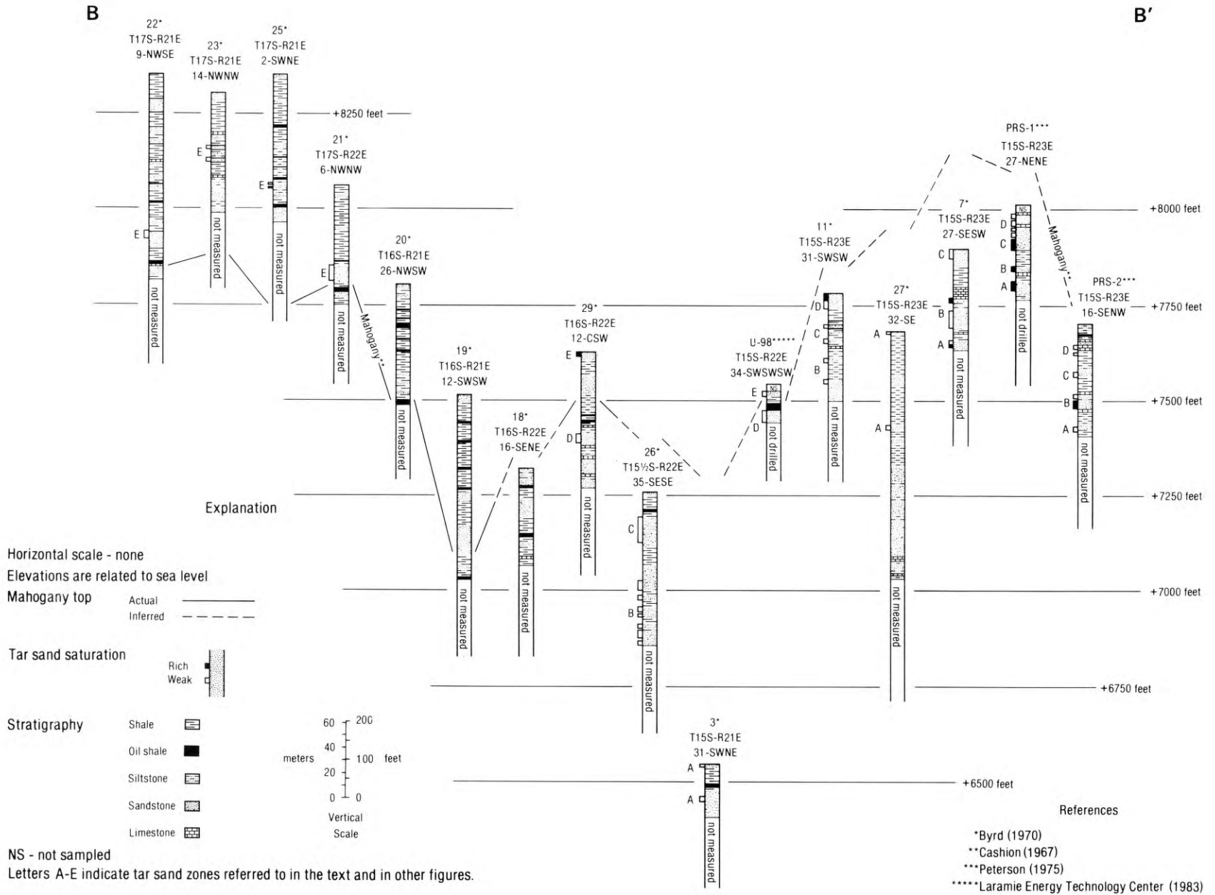
FIGURE 5. Section B-B' — Correlation of measured sections and drill holes to top of Mahogany oil shale and to tar sand zones (see figure 3).
