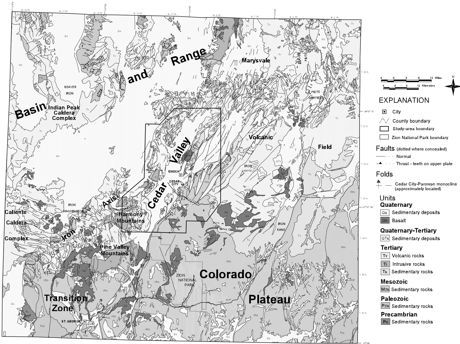
Figure 4. Tectonic map of southwestern Utah, modified from Hintze and others (2000).
