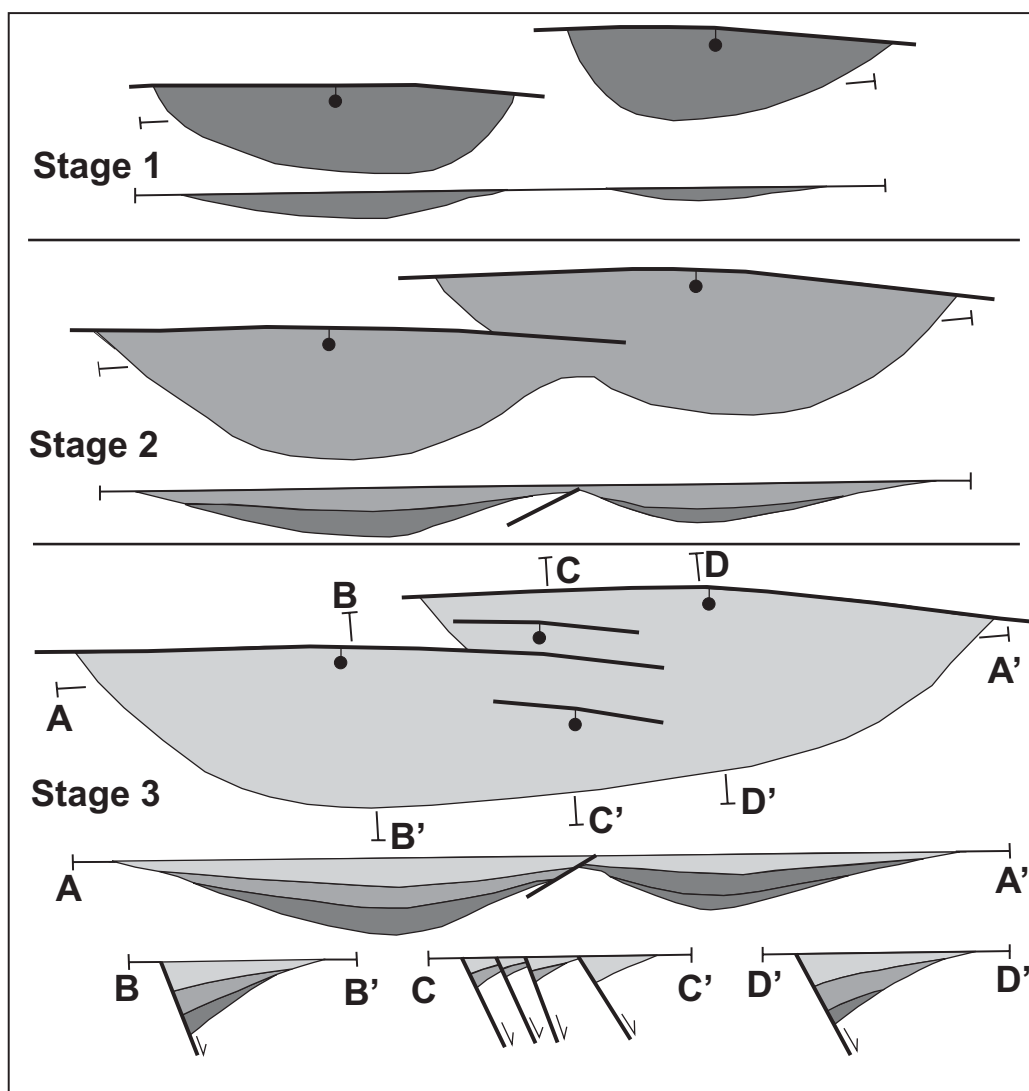
Figure 17. Basin growth and filling model for two closely overlapping fault segments. From Schlichce and Anders (1996).
