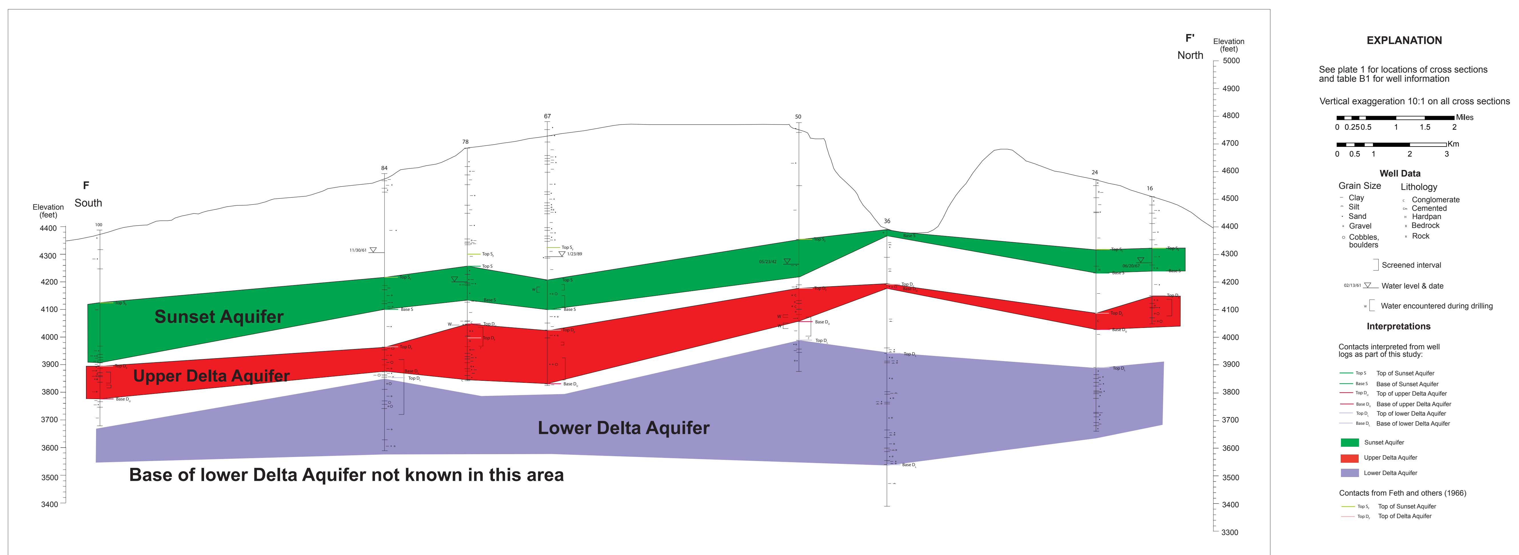
Schematic Cross Sections Through Basin Fill in the Pilot Project Study Area
