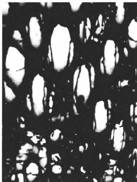
Resinite (light-colored) in cell lumens of coal from Utah.
