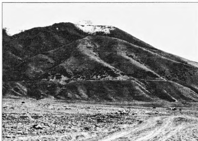
The Bonneville shoreline forms a prominent bench in the foothills of the Oquirrh Mountains near Bates Canyon in northeastern Tooele Valley. Lake Bonneville formed the shoreline between about 16,400 and 15,000 years ago (Oviatt and others, 1992).
