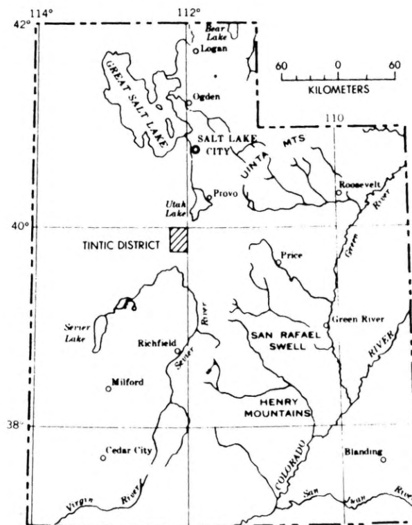
FIGURE 1.—Index map of Utah showing location of Tintic mining district.
