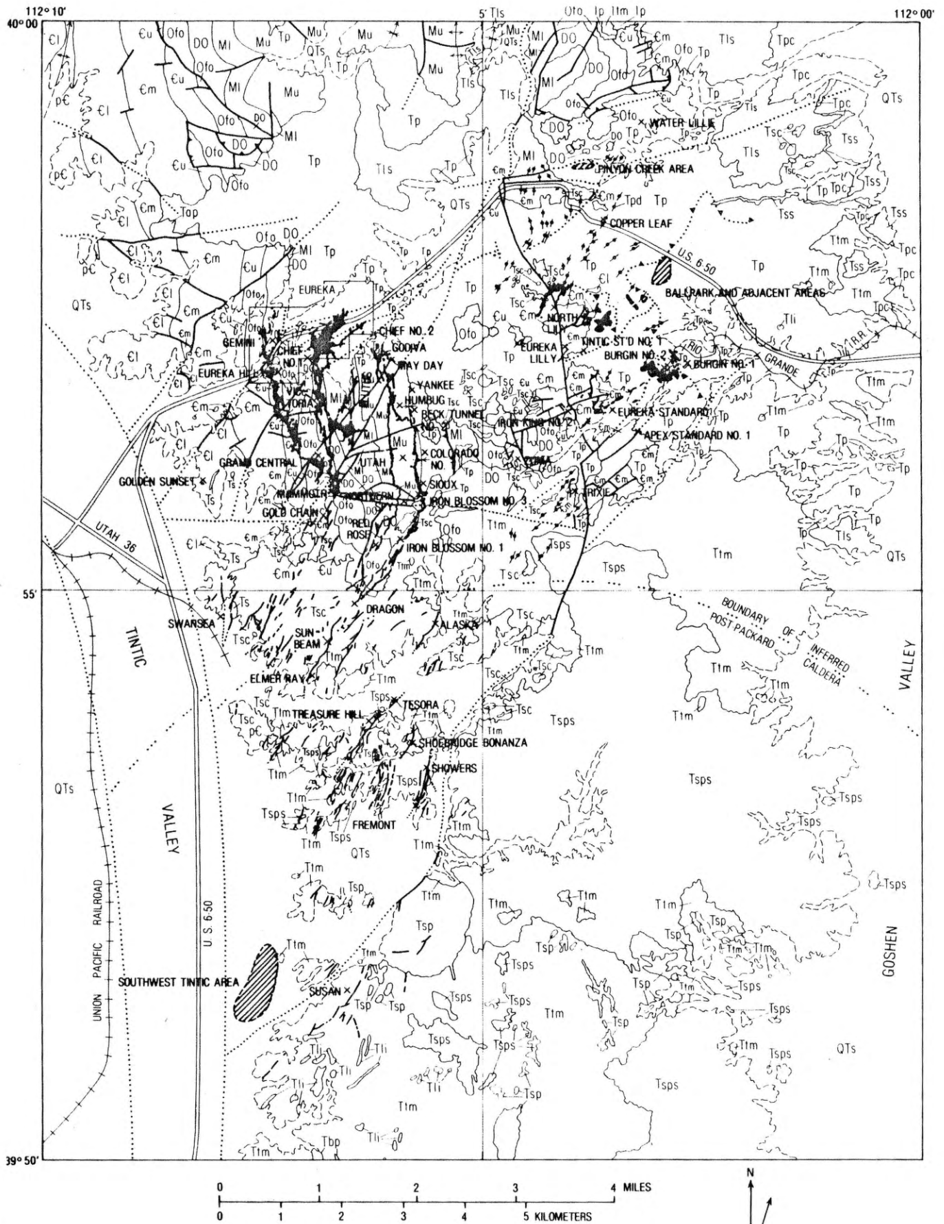
FIGURE 4.— Vertical projection of known ore bodies (solid) and mineralized areas (shaded) in the Tintic district.
